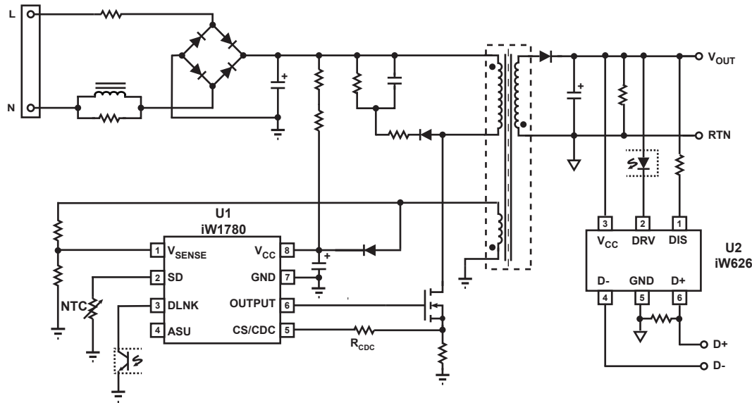
Figure 3.3 : iW1780 Typical Low Cost Application Circuit for Multi-Level Output Voltage and Current (Using iW626 as Secondary-Side Controller for QC2.0. Achieving < 50mW No-Load Power Consumption Without Using Active Start-up Device.)
