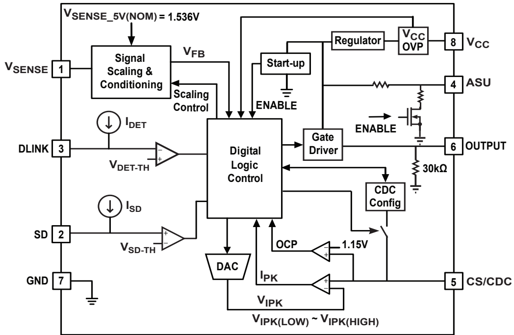
Figure 8.1 : iW1780 Functional Block Diagram
