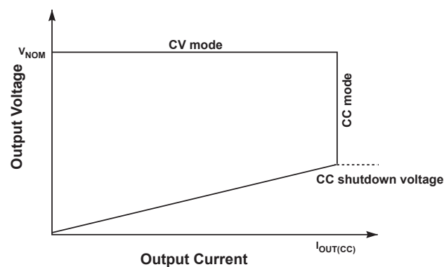
Figure 9.4 : Power Envelope
