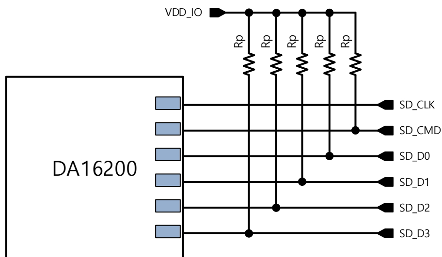
Figure 32: SDIO Pull-up Resistor
