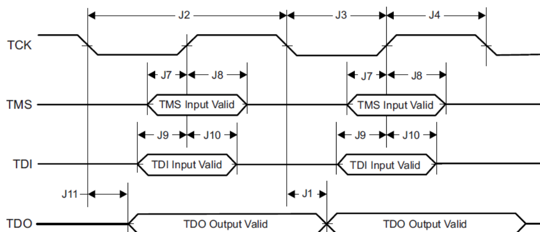
Figure 56: JTAG Timing Diagram
