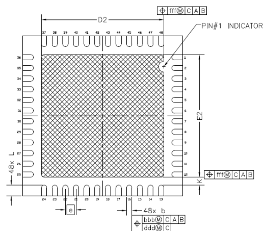
Figure 68: Bottom View
