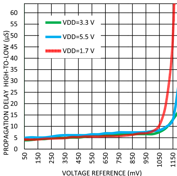
Figure 35. Maximum Propagation Delay High-to-Low vs. Voltage Reference at Room Temperature, Vod = 2 mV.
