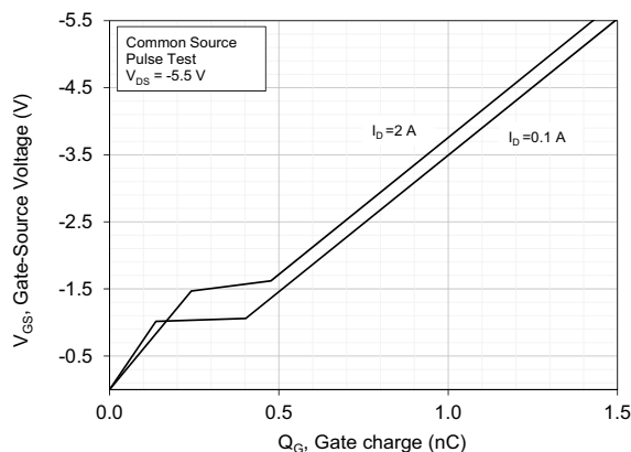
Figure 122: Typical Gate Charge vs. Gate-Source Voltage
