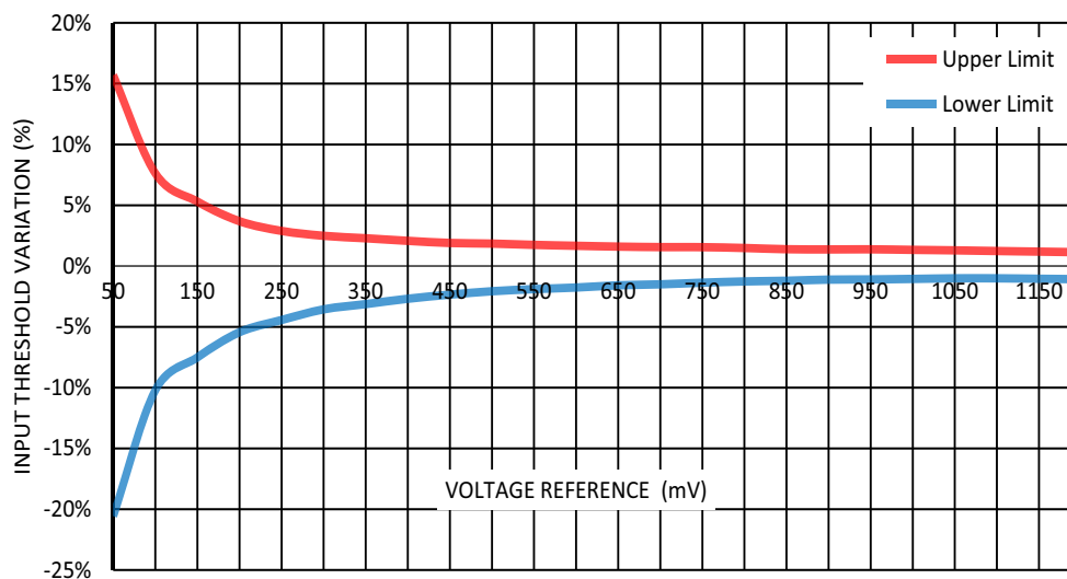
Figure 48: Typical Input Threshold Variation (Including Vref Variation, ACMP Offset) vs. Voltage Reference
