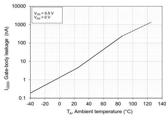
Figure 118: Gate-Body Leakage vs. Ambient Temperature
