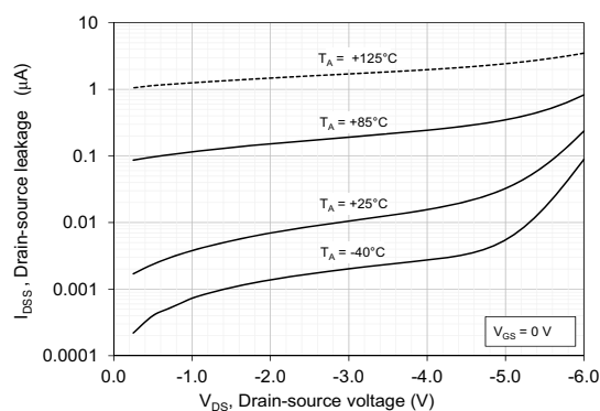
Figure 117: Zero Gate Voltage Drain Current
