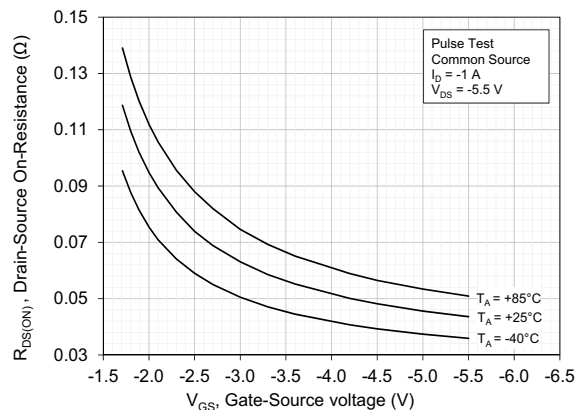
Figure 112: Gate-Source On-Resistance Gate-Source Voltage
