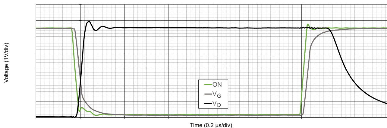
Figure 106: Typical Switching Waveforms (Internal Drive, Resistive Load, R_L = 100 \Omega , V_{DD} = V_{IN} = 5.5 \text{ V} )
