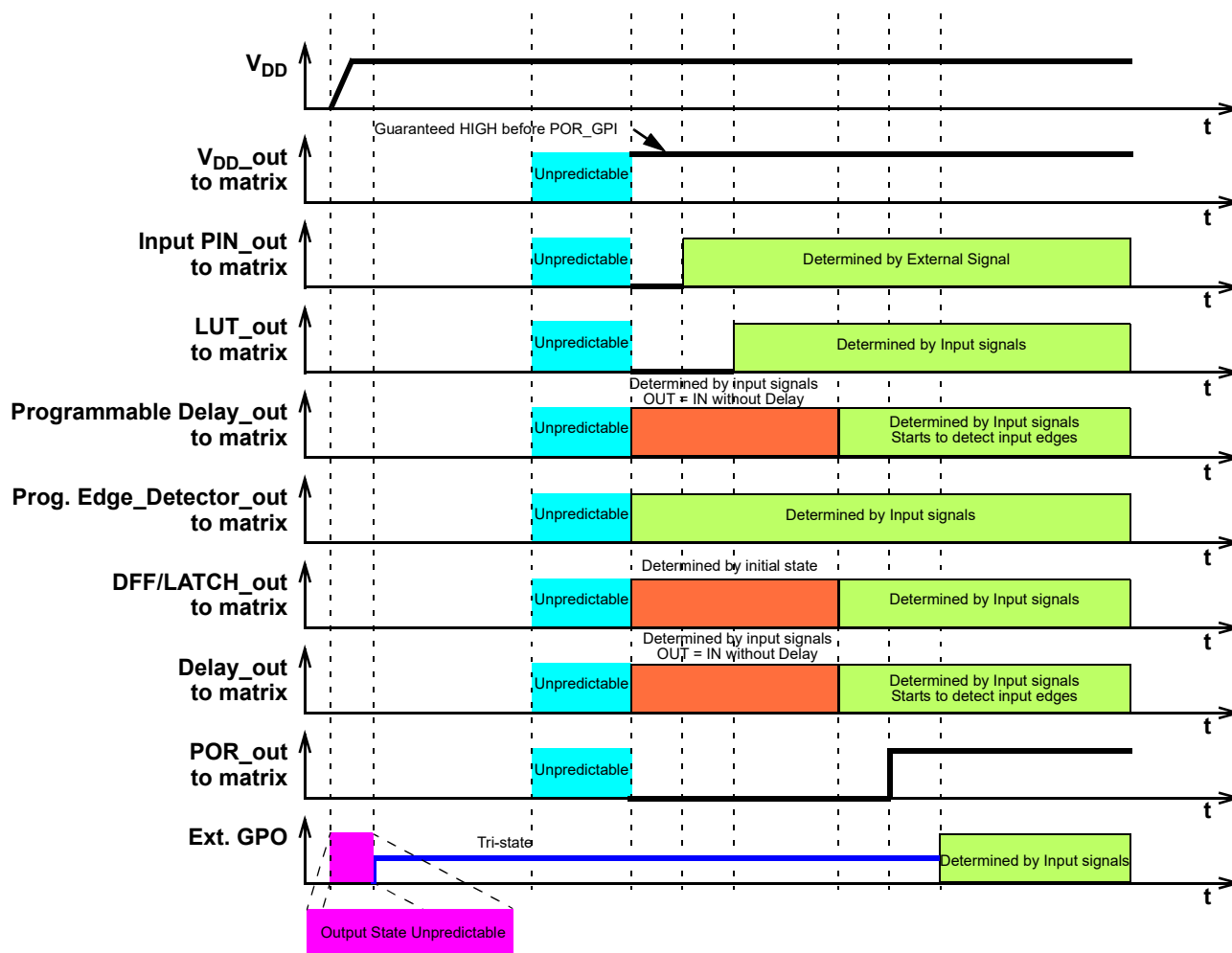
Figure 72: Internal Macrocell States during POR Sequence
