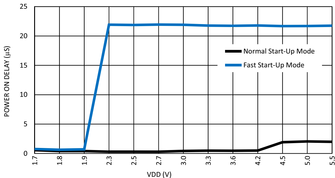
Figure 64: Oscillator Maximum Power-On Delay vs. V_{DD} at T = 25\text{ }^{\circ}\text{C} , OSC0 = 25 kHz
