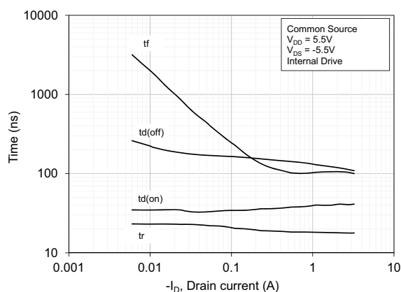
Figure 120: Typical Switching Time (Internal Gate Drive) at V_{DS} = 5.5\text{ V}
