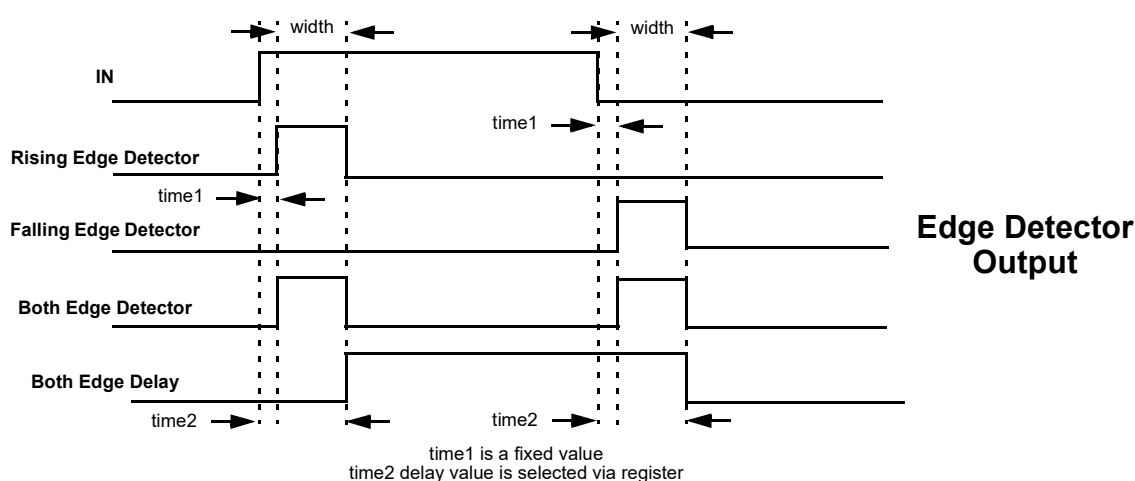
Figure 54: Edge Detector Output
