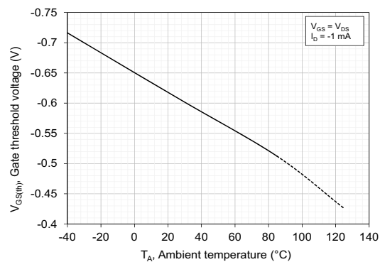
Figure 116: Gate Threshold Voltage vs Ambient Temperature
