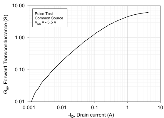
Figure 114: Typical Forward Transconductance
