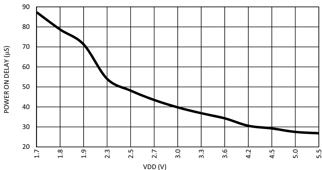
Figure 65: Oscillator Maximum Power-On Delay vs. V_{DD} at T = 25\text{ }^{\circ}\text{C} , OSC1 = 25 MHz
