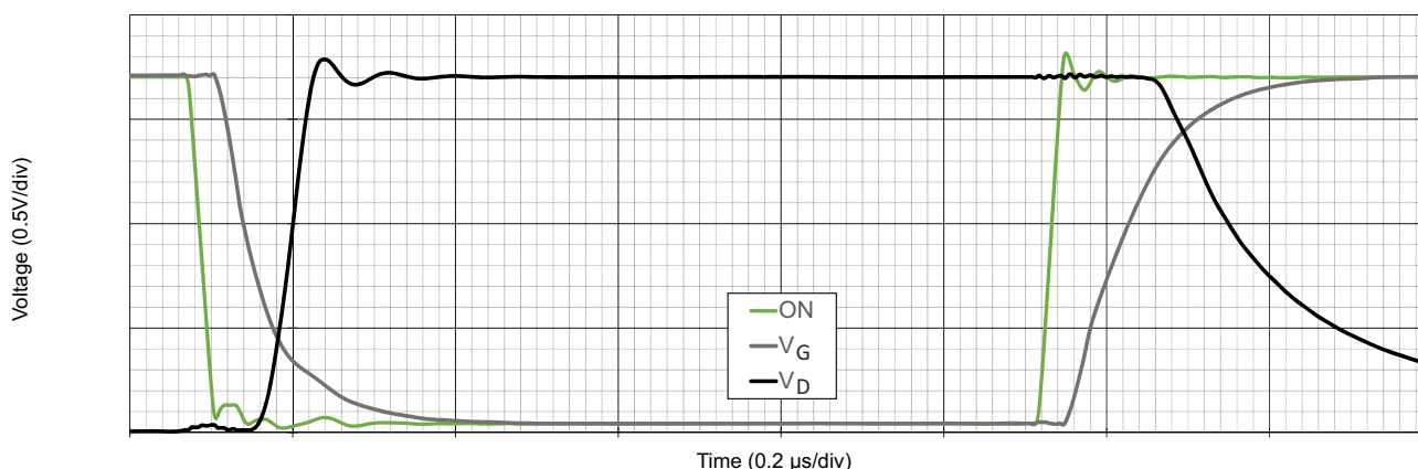
Figure 107: Typical Switching Waveforms (Internal Drive, Resistive Load, R_L = 100 \Omega , V_{DD} = V_{IN} = 1.71 \text{ V} )
