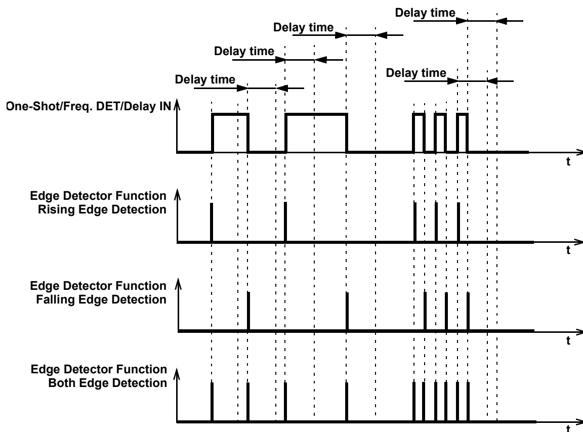
Figure 34: Edge Detection Mode Timing Diagram
