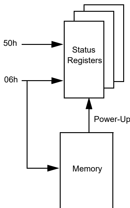
Figure 23: AT25XE161D Register Structure
