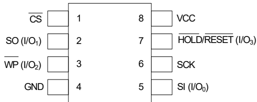
8S1 8-lead SOIC Package (0.150") 8S2 8-lead EIAJ SOIC Package (0.208") (Top View)
