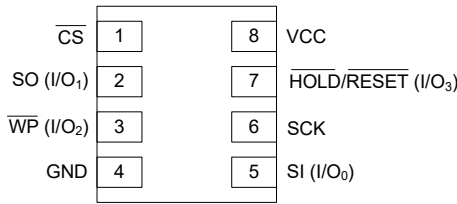
8MA3 8-pad Ultra-Thin DFN Package 2 x 3 x 0.6 mm (Top View)
