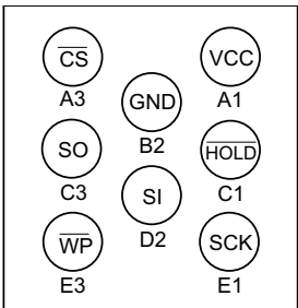
8-ball WLCSP Package 3 x 2 x 3 ball matrix (bottom view)
