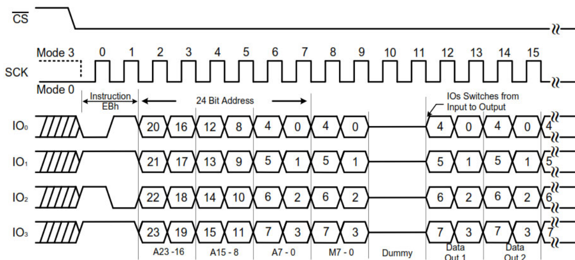
Figure 8-20. Fast Read Quad I/O Instruction (Initial instruction or previous M7-0 \neq Axx, QPI mode, 80 MHz)
