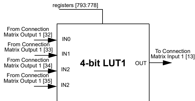
Figure 34: 4-bit LUT_1
