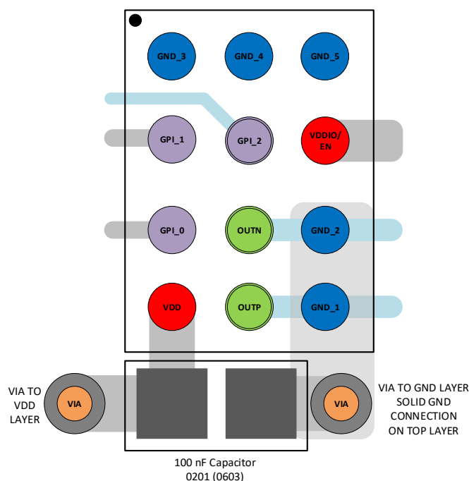
Figure 15: WLCSP Example PCB Layout
