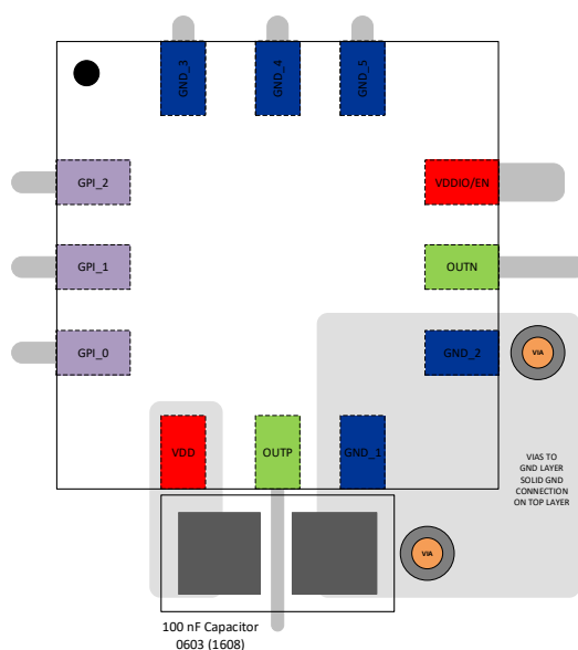
Figure 16: QFN Example PCB Layout
