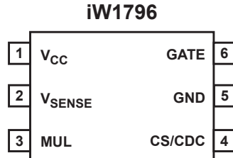
Figure 4.1 : 6-Lead SOT23-6 Package
