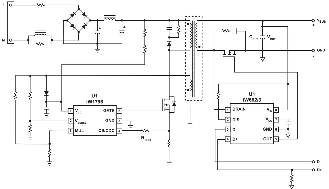
Figure 3.1 : iW1796 Typical Application Circuit for Multi-Level Output Voltage and Current (Using iW662/3 as Secondary-Side Controller for Rapid Charge Protocols. Achieving < 75mW No-Load Power Consumption (with ample margin) in Typical 15W Design.)
