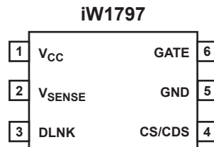
Figure 4.1 : 6-Lead SOT23-6 Package
