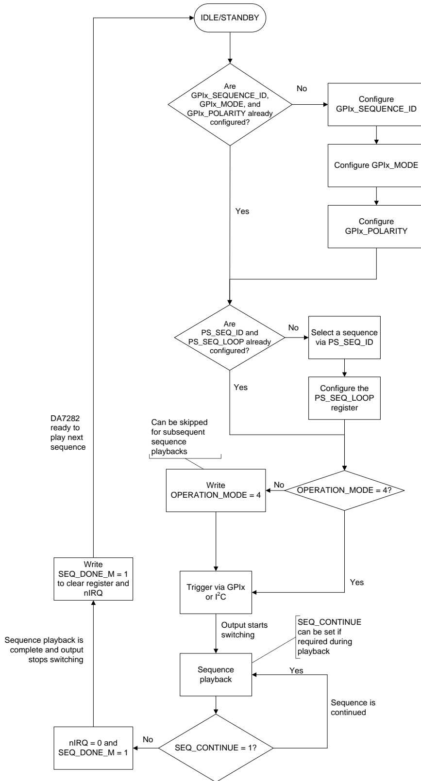
Figure 17: Operation in ETWM Mode
