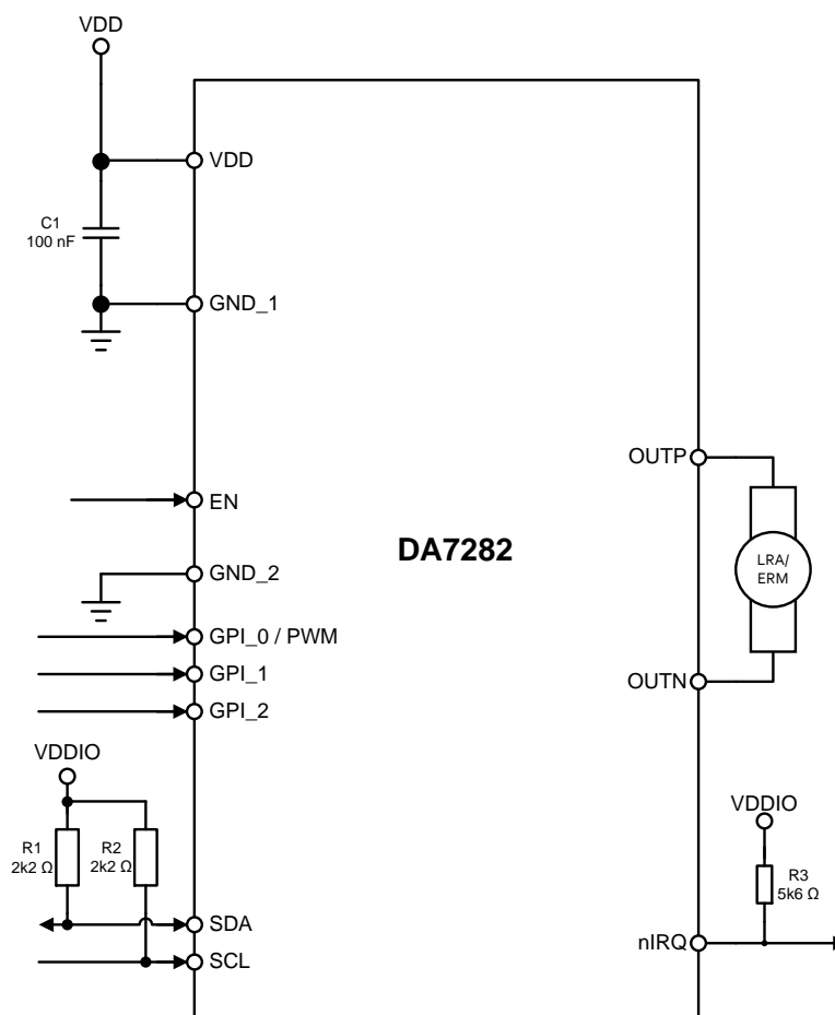
Figure 43: External Components Diagram
