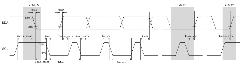
Figure 5: I 2 C Interface Timing
