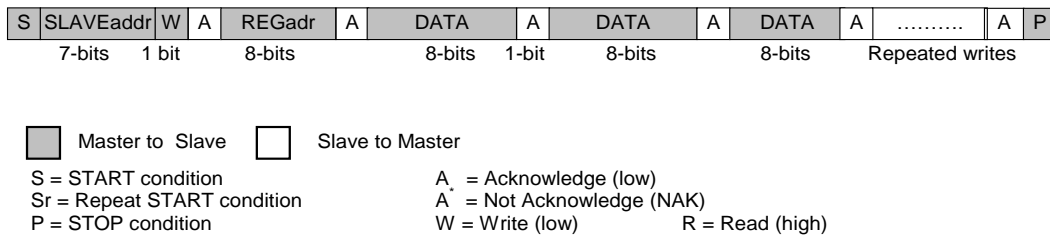
Figure 39: I 2 C Page Write (SDA line)
