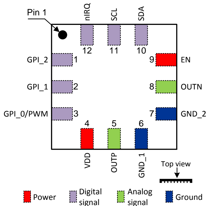
Figure 4: DA7282 QFN Pinout Diagram (Top View)
