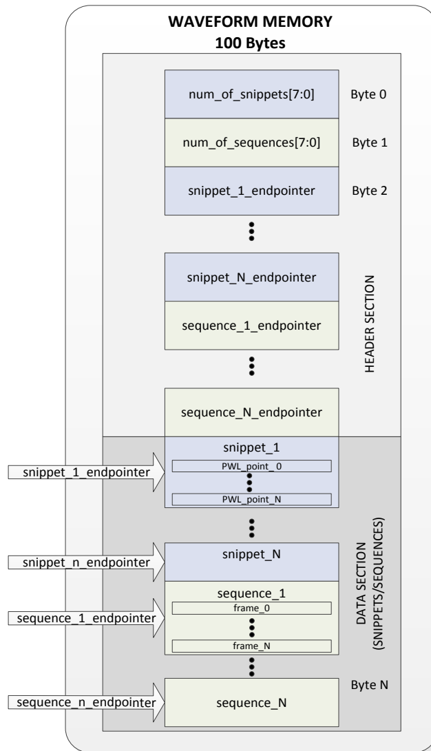
Figure 26: Waveform Memory Structure
