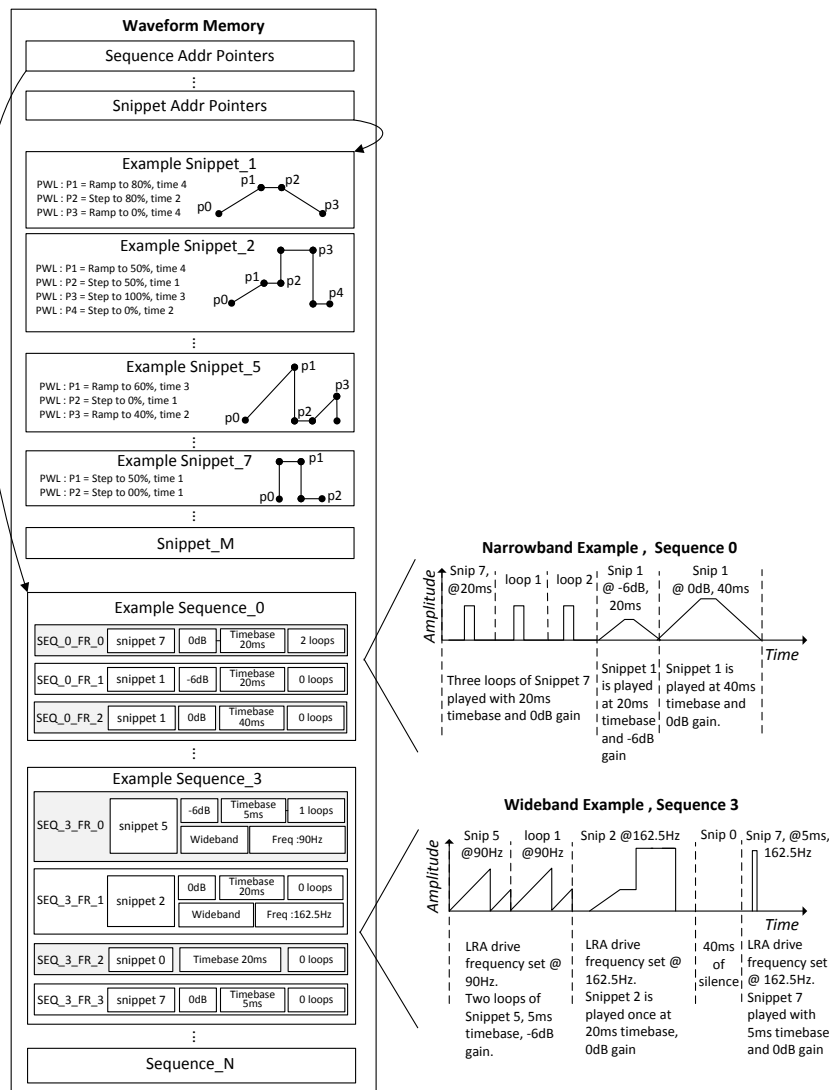
Figure 31: Waveform Memory Example
