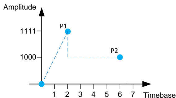
Figure 27: Snippet Ramp and Step with ACCELERATION_EN = 1
