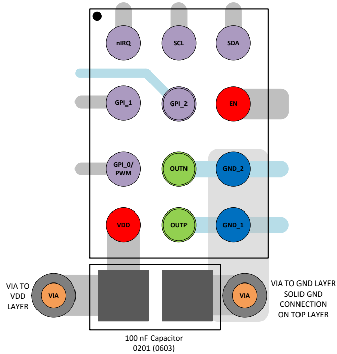
Figure 44: WLCSP Example PCB Layout
