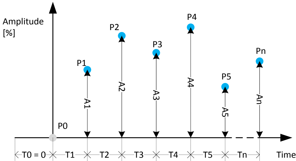
Figure 28: Snippet Example
