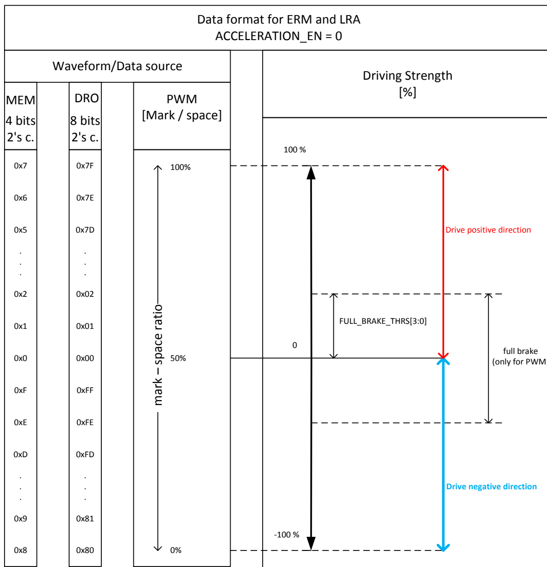
Figure 32: Overview of Data Formats with Acceleration Disabled
