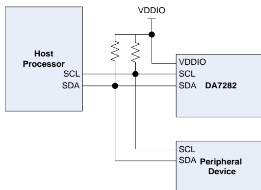
Figure 34: Schematic of the I 2 C Control Interface Bus
