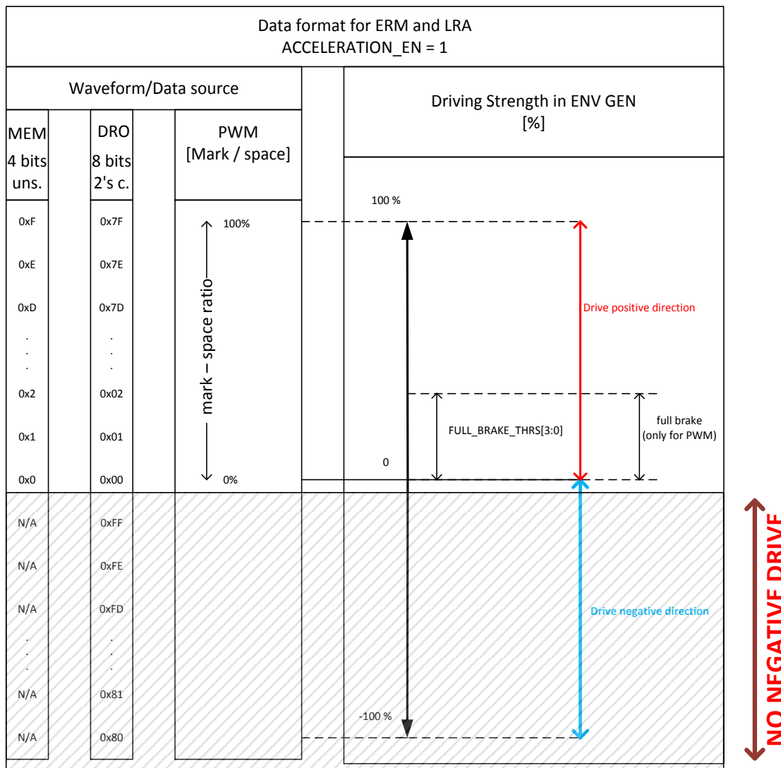
Figure 33: Overview of Data Formats with Acceleration Enabled
