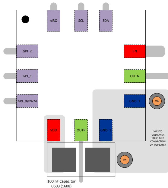
Figure 45: QFN Example PCB Layout
