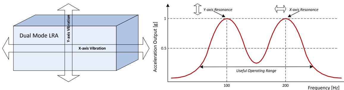
Figure 8: Dual Mode LRA Response across Frequency
