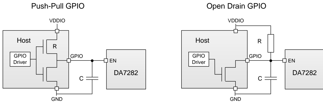
Figure 25: EN Pin Control in Push-Pull Configuration (Left) and Open Drain Configuration (Right)
