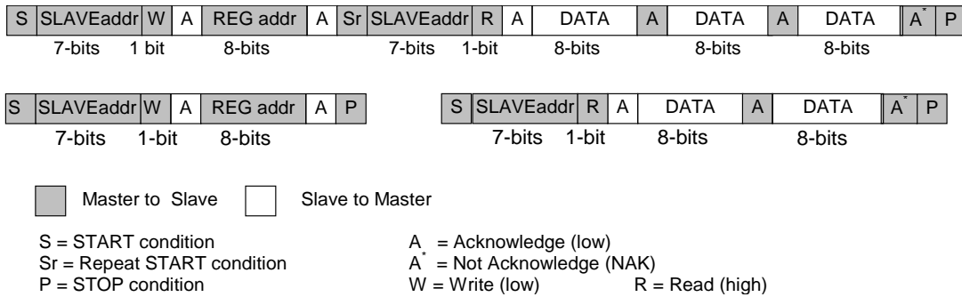
Figure 38: Examples of I 2 C Page Read (SDA line)
