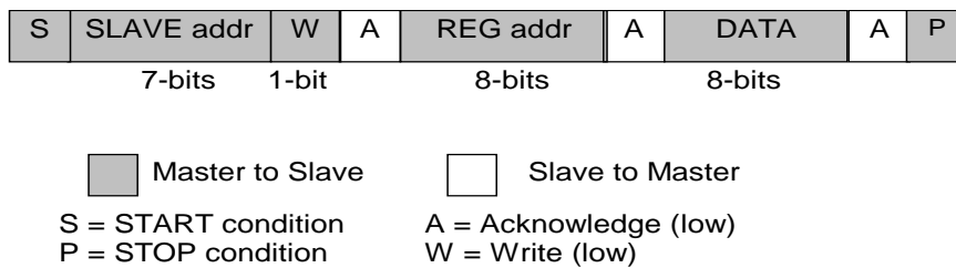
Figure 36: I 2 C Byte Write (SDA line)
