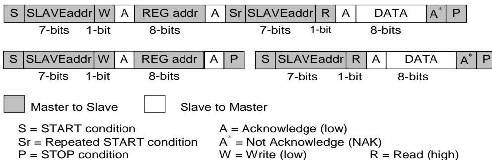
Figure 37: Examples of the I 2 C Byte Read (SDA line)
