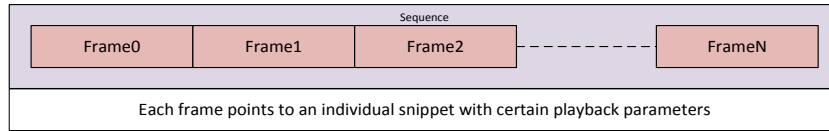
Figure 30: Sequence Structure
