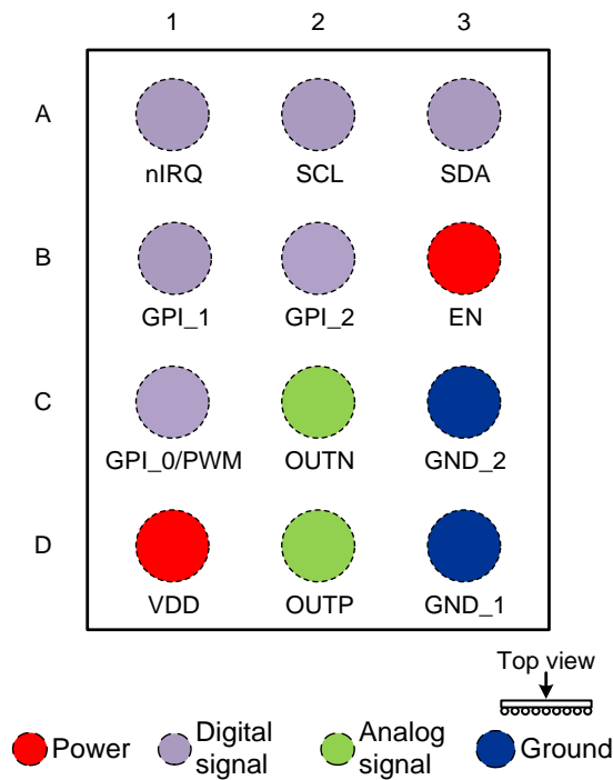
Figure 3: DA7282 WLCSP Pinout Diagram (Top View)
