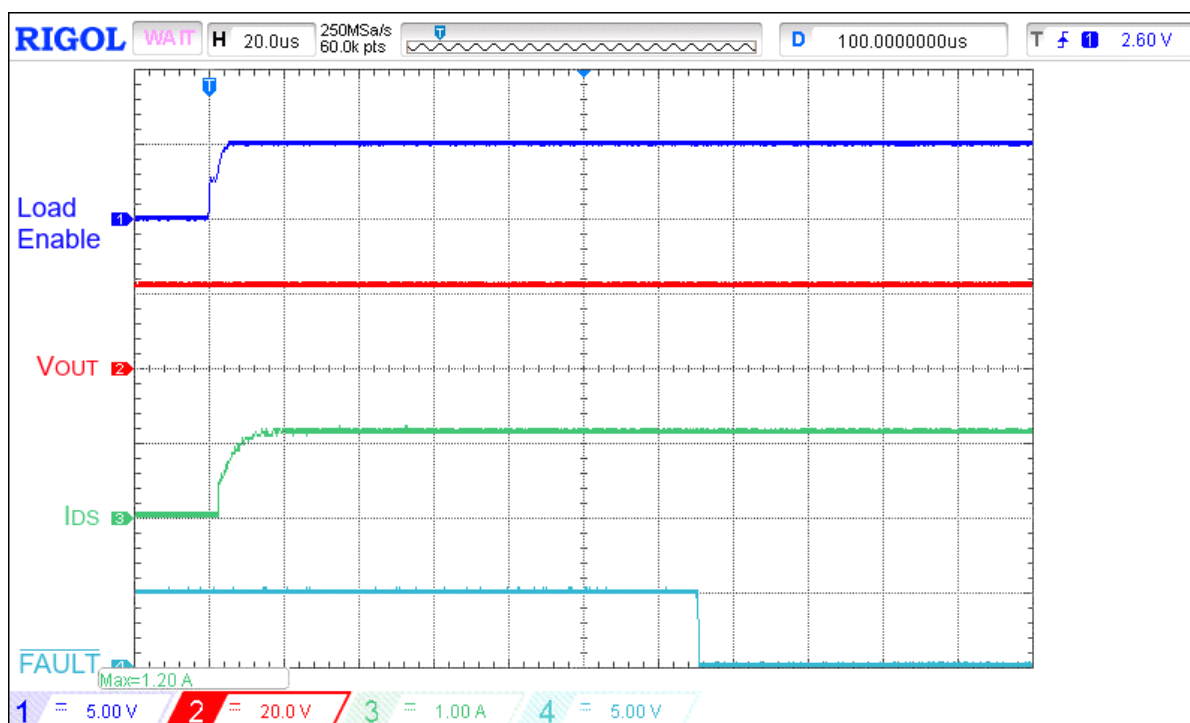
Figure 12. Typical FAULT assertion waveform for V IN = 24 V, C LOAD = 10 \mu F, I ACL = 1 A, R SET = 91 k \Omega , switch on 18.5 \Omega load
