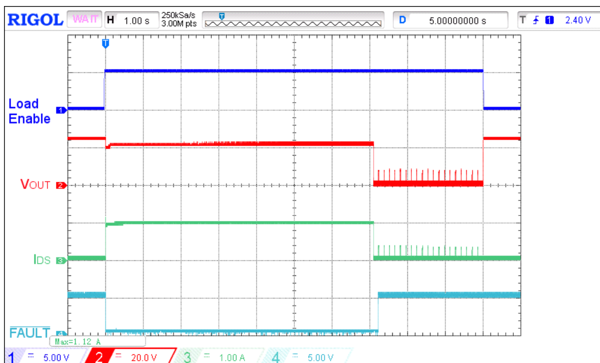
Figure 11. Thermally induced SOA shutdown for V IN = 24 V, C LOAD = 10 \mu F, I ACL = 1 A, R SET = 91 k \Omega
