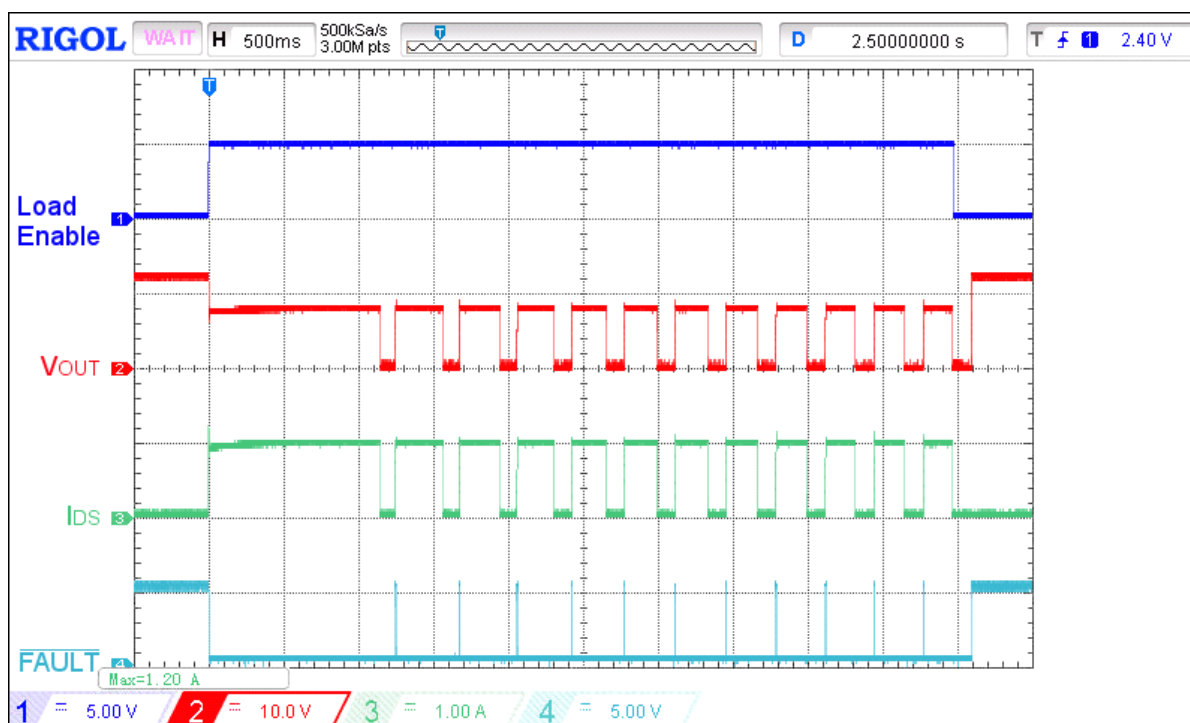
Figure 10. Typical ACL operation waveform for V IN = 12 V, C LOAD = 10 \mu F, I ACL = 1 A, R SET = 91 k \Omega
