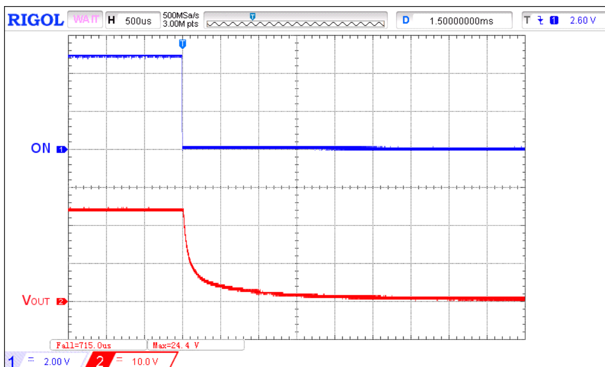
Figure 9. Typical Turn OFF operation waveform for V IN = 24 V, C SLEW = 10 nF, C LOAD = 10 \mu F, R LOAD = 100 \Omega
