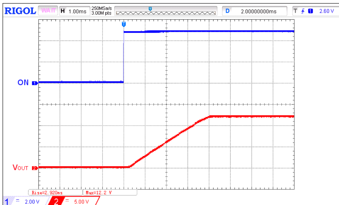
Figure 2. Typical Turn ON operation waveform for V IN = 12 V, C SLEW = 10 nF, C LOAD = 10 \mu F, R LOAD = 100 \Omega
