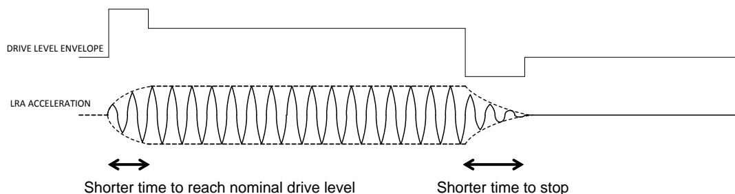
Figure 12: LRA Single Step with Acceleration and Rapid Stop
