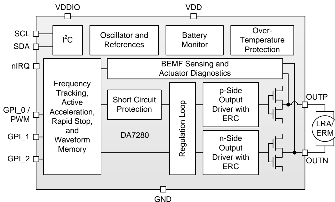
Figure 2: DA7280 Block Diagram
