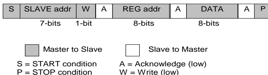
Figure 35: I 2 C Byte Write (SDA line)
