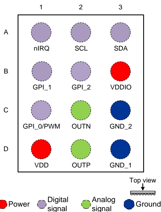
Figure 3: DA7280 WLCSP Pinout Diagram (Top View)
