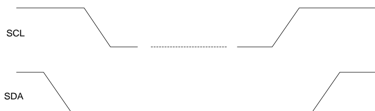
Figure 34: I 2 C START and STOP Conditions
