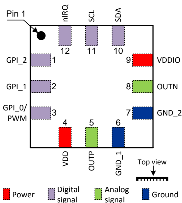
Figure 4: DA7280 QFN Pinout Diagram (Top View)
