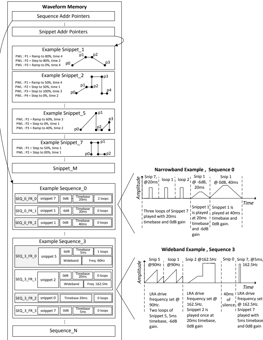
Figure 30: Waveform Memory Example
