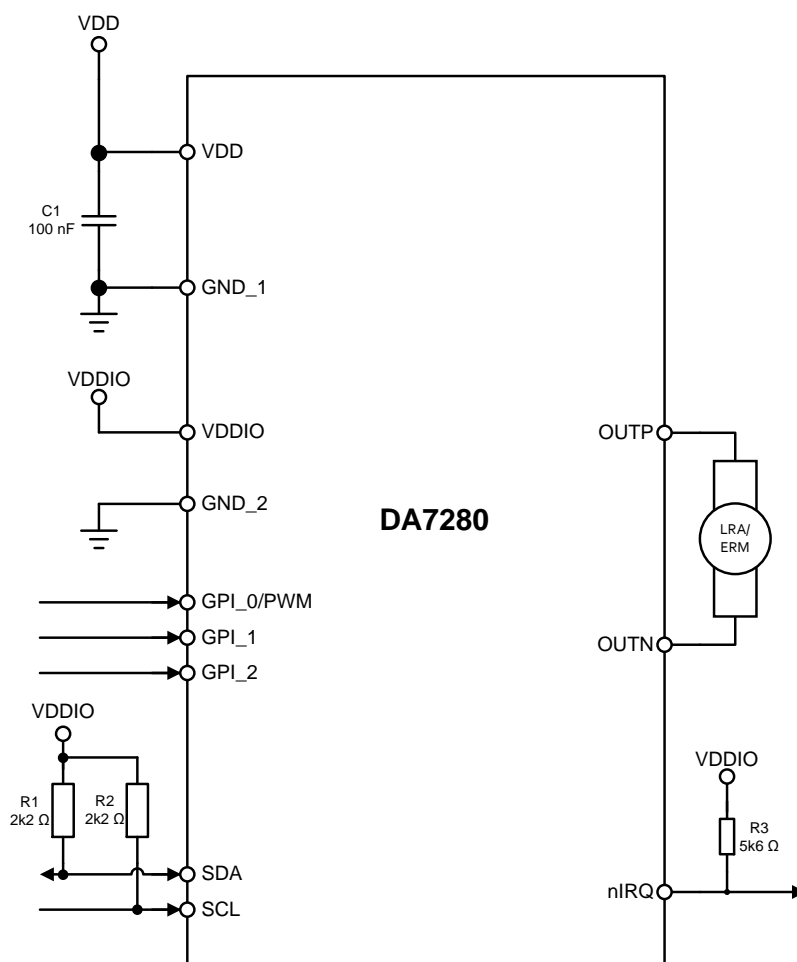
Figure 42: External Components Diagram
