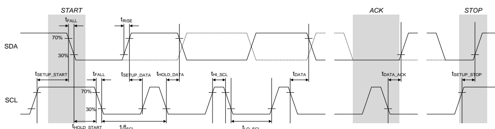
Figure 5: I 2 C Interface Timing
