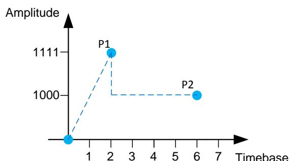
Figure 26: Snippet Ramp and Step with ACCELERATION_EN = 1
