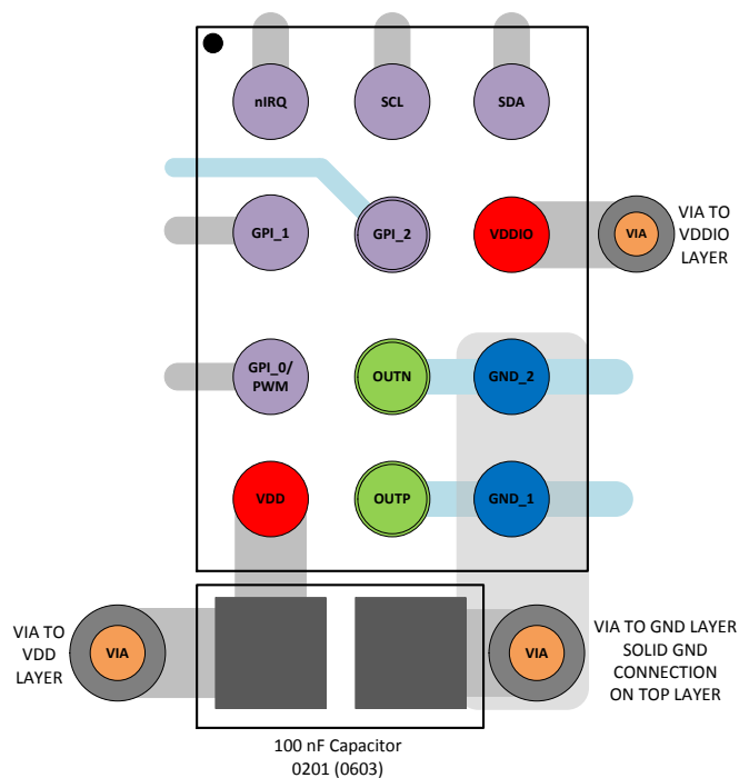
Figure 43: WLCSP Example PCB Layout
