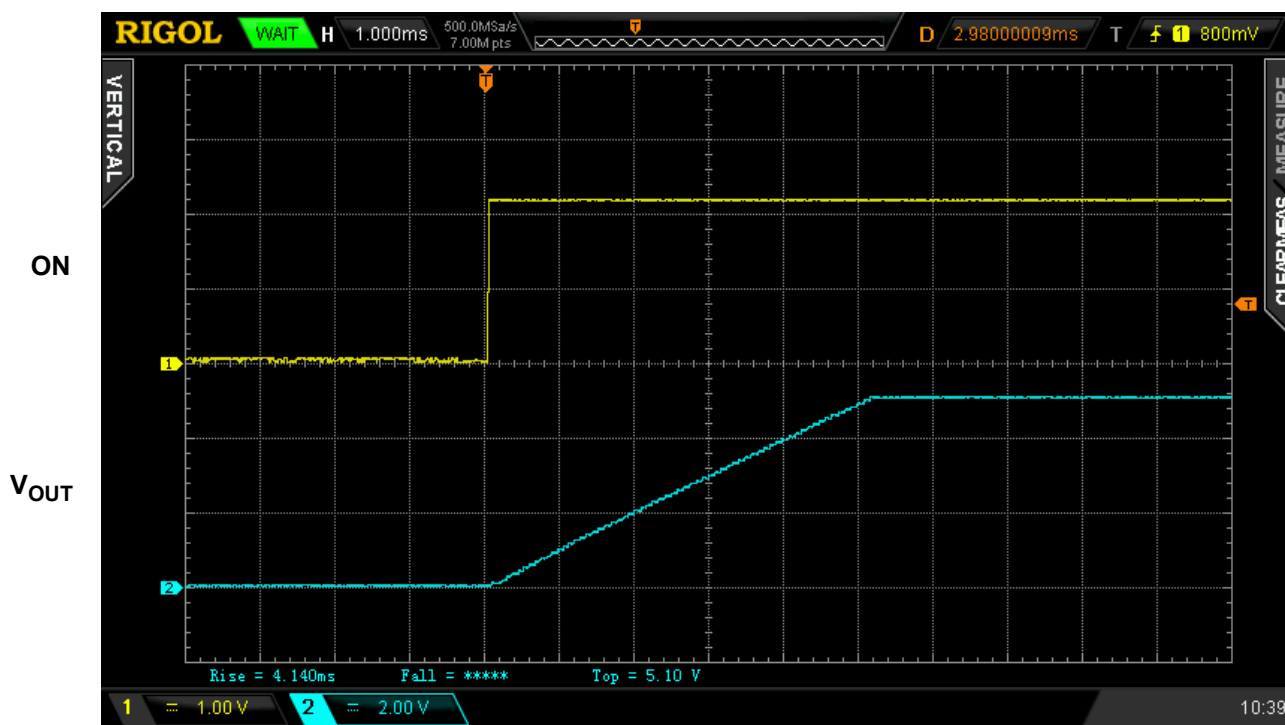
Figure 1. Typical Turn ON operation waveform for V_{DD} = V_{IN} = 5\text{ V} , C_{SLEW} = 12\text{ nF} , C_{LOAD} = 10\text{ }\mu\text{F} , R_{LOAD} = 20\text{ }\Omega
