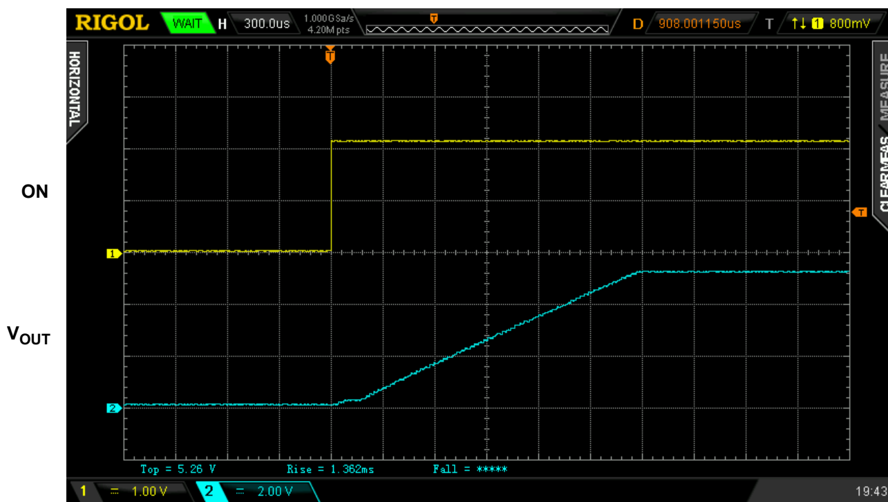
Figure 2. Typical Turn ON operation waveform for V_{DD} = V_{IN} = 5\text{ V} , C_{SLEW} = 4\text{ nF} , C_{LOAD} = 10\text{ }\mu\text{F} , R_{LOAD} = 20\text{ }\Omega
