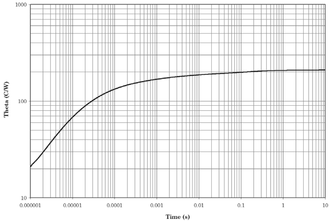
FIGURE 4. Thermal impedance graph ( R_{\theta\text{JSP}} ) for 2N2857UB.
