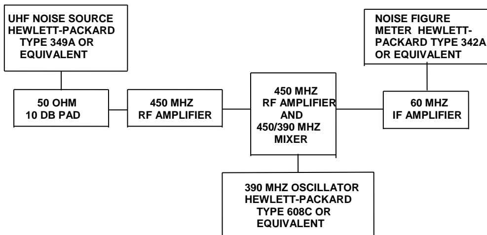
FIGURE 7. Block diagram for noise figure test.
