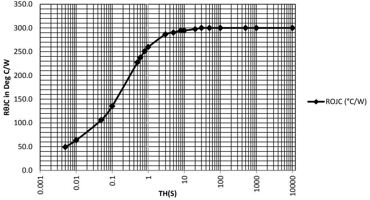
* FIGURE 6. Thermal impedance graph TO-72 ( R_{\theta JC} ) for 2N2857.
