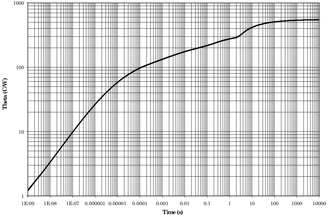
* FIGURE 5. Thermal impedance graph TO-72 ( R_{\theta JA} ) for 2N2857.
