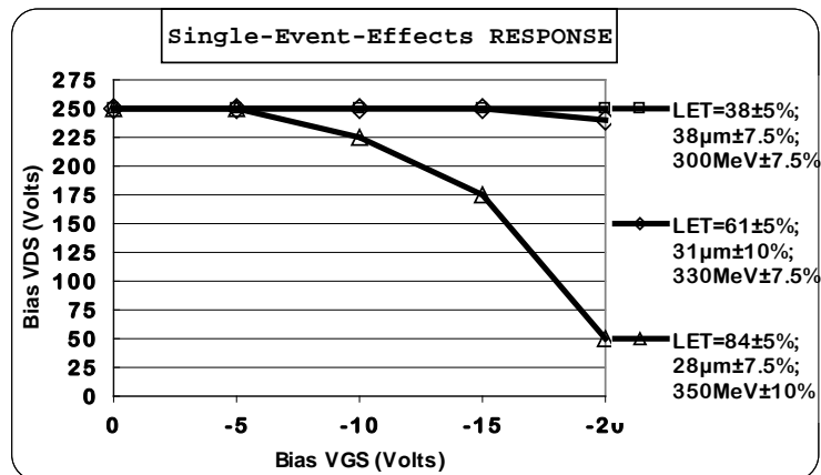
* FIGURE 5. Typical SEE safe operating area graphs.
