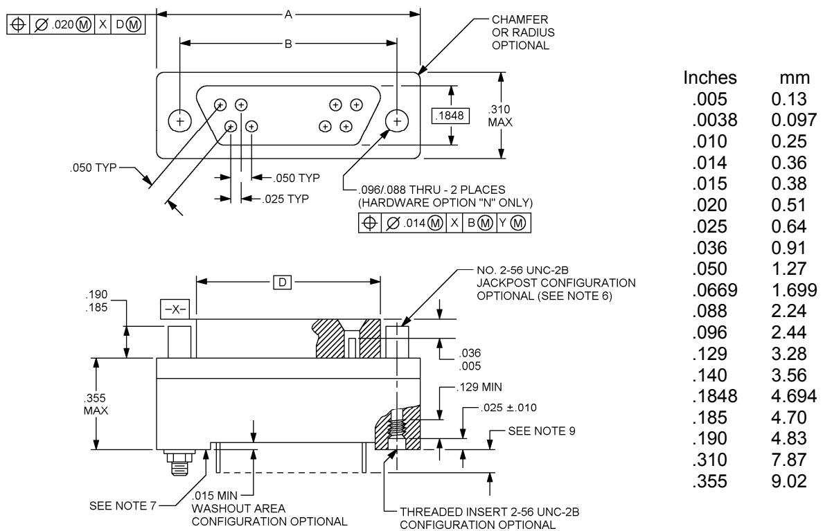
FIGURE 1. Connector plug.
