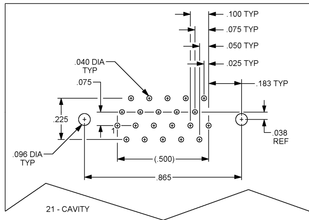
FIGURE 3. Layout arrangement.
