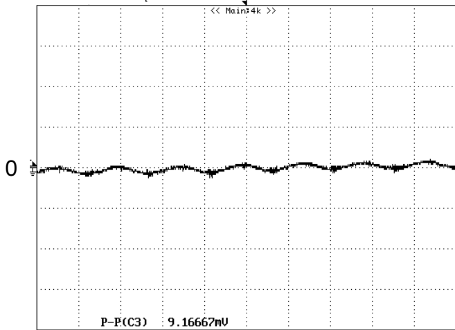
Figure 12: Input reflected ripple current, i_s , through a 12 \mu H source inductor at nominal input voltage and rated load current (20 mV/div, 20 ns/div)
