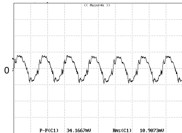
Figure 14: Output voltage ripple at nominal input voltage and rated load current ( I_o=5A ) (20 mV/div, 20 ns/div) Load capacitance: 1 \mu F ceramic capacitor and 10 \mu F tantalum capacitor. Bandwidth: 20 MHz. Scope measurements should be made using a BNC cable (length shorter than 20 inches). Position the load between 51 mm to 76 mm (2 inches to 3 inches) from the module
