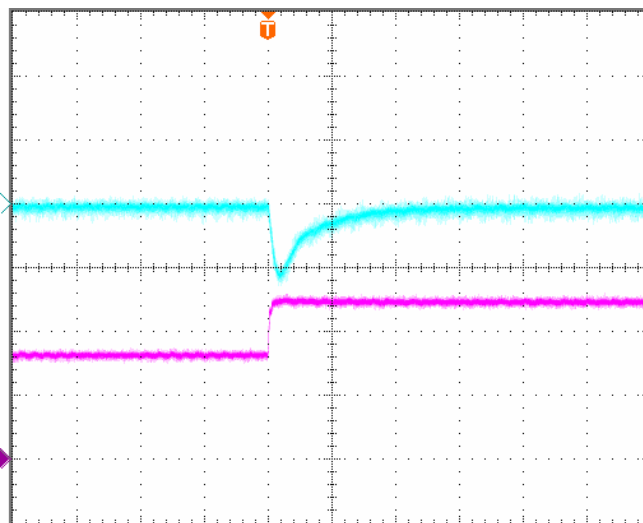
Figure 9: Output voltage response to step-change in load current (50%-75% of I_o , max; di/dt = 1A/\mu s ). Load cap: 400\mu F , ceramic capacitor. Top Trace: V_{out} (100mV/div, 200us/div); Bottom Trace: output current (1.5A/div, 200us/div)
