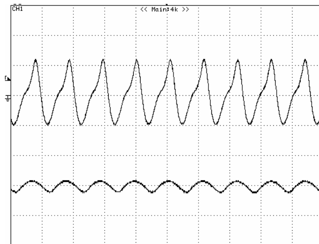
Figure 11: Top trace: Input Terminal Ripple Current, i_c , at full rated output current and nominal input voltage with 12\mu H source impedance and 100\mu F electrolytic capacitor (2A/div, 2us/div), Setup is shown in Figure 10 top picture.
