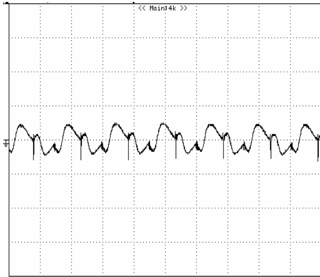
Figure 14: Output voltage ripple at nominal input voltage and rated load current ( I_o=12A ) (20 mV/div, 2 μs/div) Load capacitance: 1 μF ceramic capacitor and 10 μF tantalum capacitor. Bandwidth: 20 MHz. Scope measurements should be made using a BNC cable (length shorter than 20 inches). Position the load between 51 mm to 76 mm (2 inches to 3 inches) from the module
