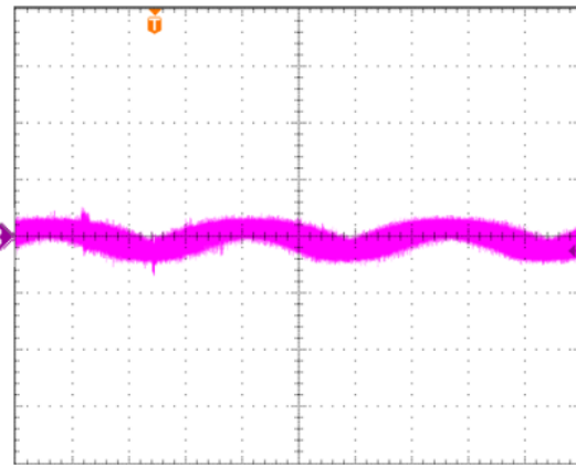
Figure 22: Input Reflected Ripple Current, i_s , through a 12\mu H source inductor at 48Vdc input voltage, 5Vdc output voltage and max load current (100mA/div, 1us/div).
