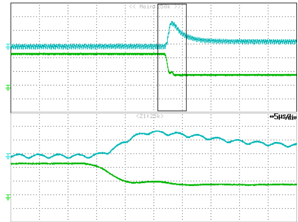
Figure 19: Transient Response
