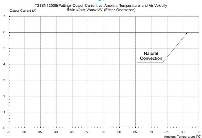
Figure 36: Output current vs. ambient temperature and air velocity @ V_{in}=24V , V_{out}=12V (Either Orientation, Potting)
