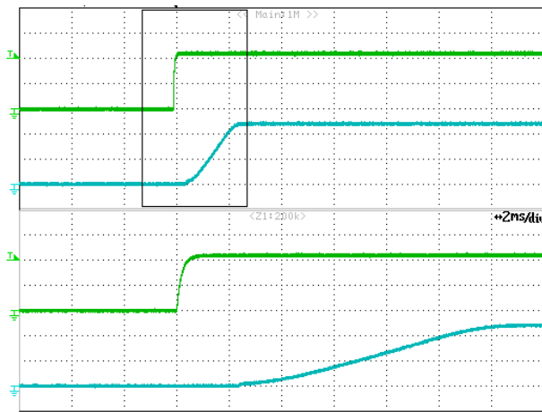
Figure 14: Remote On/Off Start-up at open load
