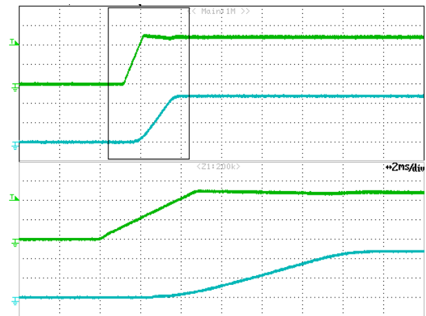
Figure 17: Input Voltage Start-up at full load
