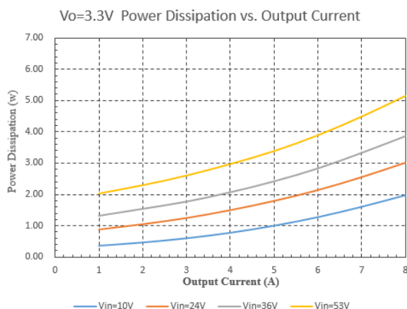
Figure 6: Power Dissipation vs. Output Current (Vo=3.3V)
