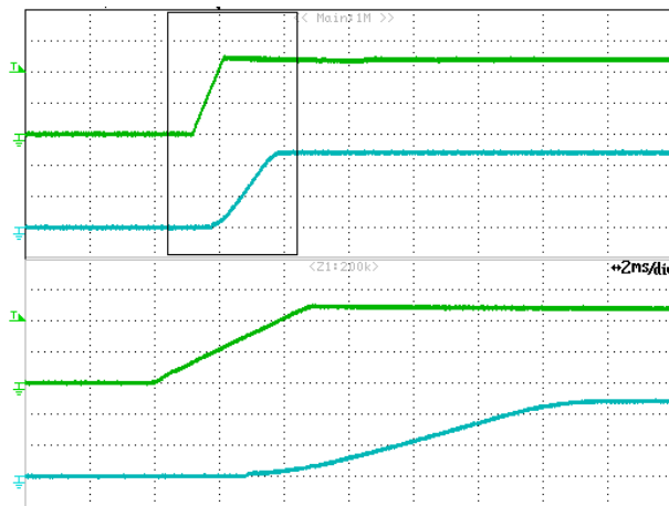
Figure 16: Input Voltage Start-up at open load
