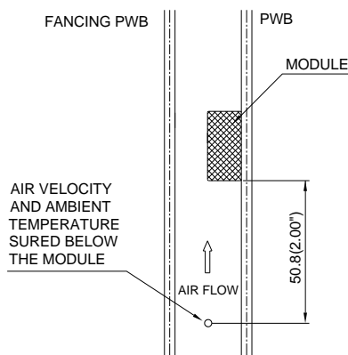
Figure 27: Wind Tunnel Test Setup
