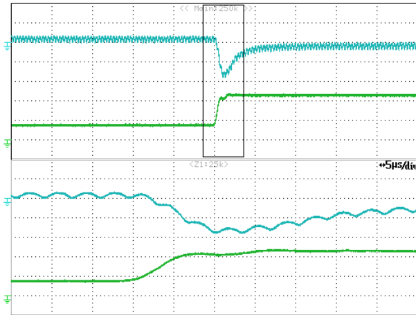
Figure 18: Transient Response
