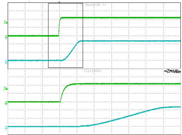
Figure 15: Remote On/Off Start-up at full load
