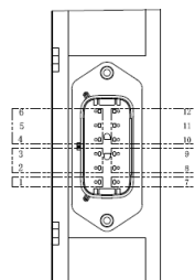
PIN CONNECTIONS:
