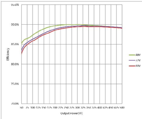
Figure 1: Efficiency vs. Output Power @ V_{in}=48V, 72V, 80V
