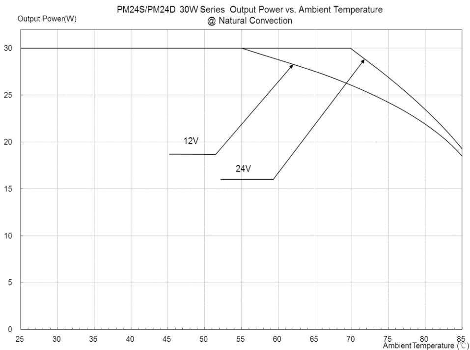
Figure1: PM24S/PM24D 30W series Output power vs Ambient temperature@Natural convection
