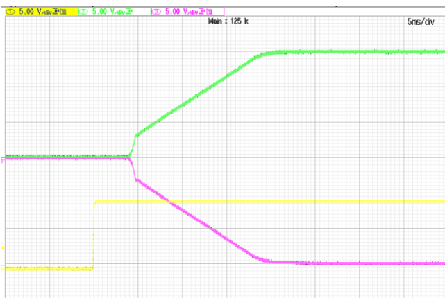
Turn-on transient at full load current (5ms/div). Top two traces: Vout; 5V/div; Bottom Trace: ON/OFF input: 5V/div.
