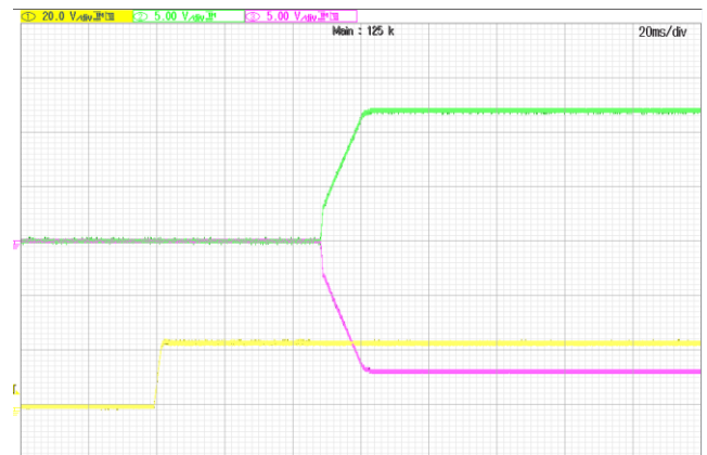
Turn-on transient at full load current (20ms/div). Top two Traces: Vout; 5V/div; Bottom Trace: input voltage: 20V/div.
