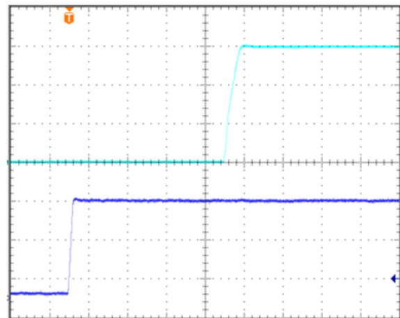
Turn-on transient at full load current (20ms/div). Top Trace: Vout; 5V/div; Bottom Trace: input voltage: 10V/div.
