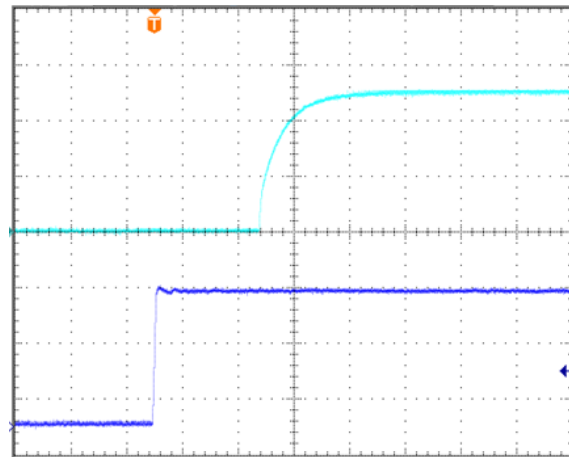
Turn-on transient at full load current (40ms/div). Top Trace: Vout; 2V/div; Bottom Trace: input voltage: 10V/div.
