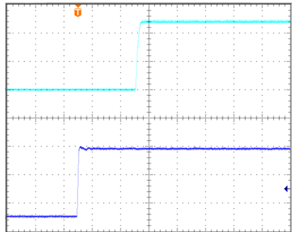
Turn-on transient at full load current (40ms/div). Top Trace: Vout; 5V/div; Bottom Trace: input voltage: 10V/div.
