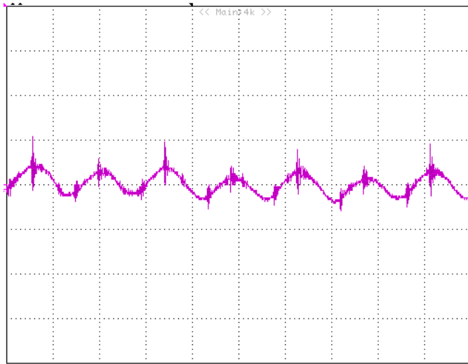
Figure 12: Input reflected ripple current, i_s , through a 12\mu\text{H} source inductor at nominal input voltage and rated load current ( 20\text{mV/div} , 2\mu\text{s/div} ).
