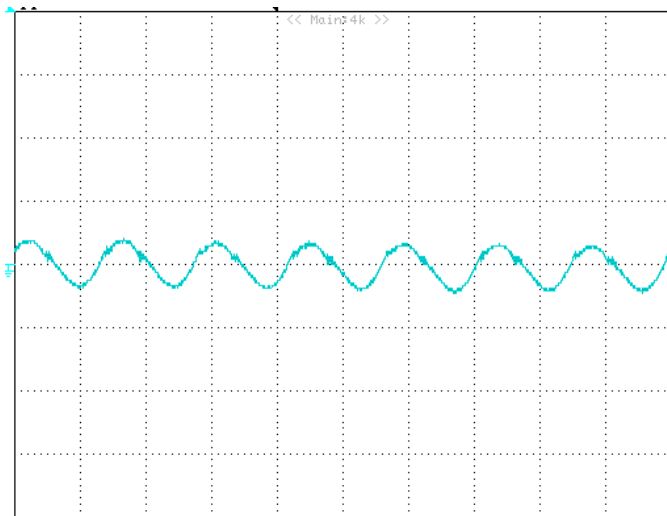
Figure 14: Output voltage ripple at nominal input voltage and rated load current ( I_o=20\text{A} ) ( 50\text{mV/div} , 2\mu\text{s/div} ) Load capacitance: 220\mu\text{F} (Electrolytic)+ 10\mu\text{F} (Tantalum)+ 1\mu\text{F} (Ceramic) and min Co. Bandwidth: 20\text{MHz} .
