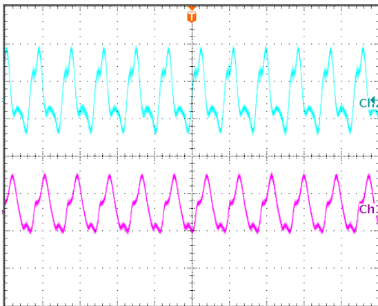
Output voltage ripple at nominal input voltage and max load current Top trace +12V, 10 mV/div, Bottom trace -12V, 20mV/div, 2μs/div. Load cap: 10μF, tantalum capacitor and 1μF ceramic capacitor. Bandwidth: 20 MHz.
