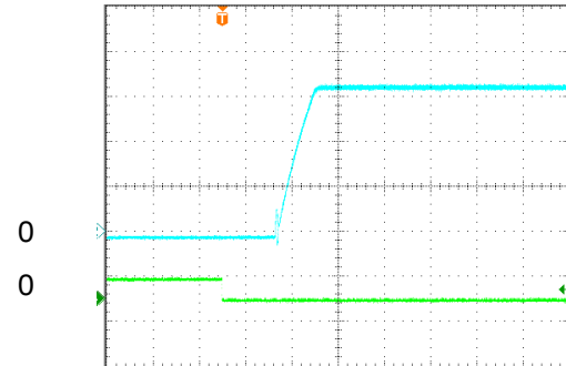
Figure 5: Turn-on transient at zero load current (10 ms/div). V_{in}=48V . Top Trace: V_{out} , 1.5V/div; Bottom Trace: ON/OFF input, 5V/div
