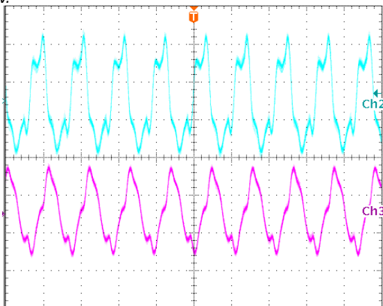
Output voltage ripple at nominal input voltage and max load current Top trace: +15V, 10 mV/div, Bottom trace: -15V, 20mV/div, 2us/div. Load cap: 10μF, tantalum capacitor and 1μF ceramic capacitor. Bandwidth: 20 MHz.
