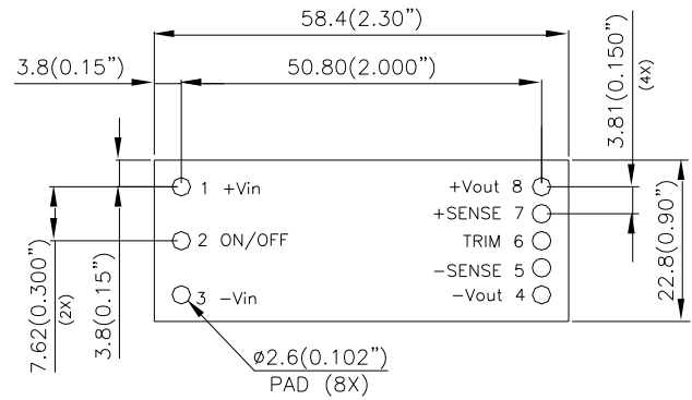
RECOMENDED P.W.B. PAD LAYOUT
