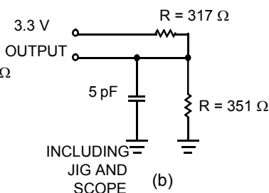
Figure 5. AC Test Loads and Waveforms
