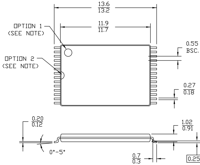
Figure 13. 28-Pin TSOP I (8 x 13.4 mm) (51-85074)
