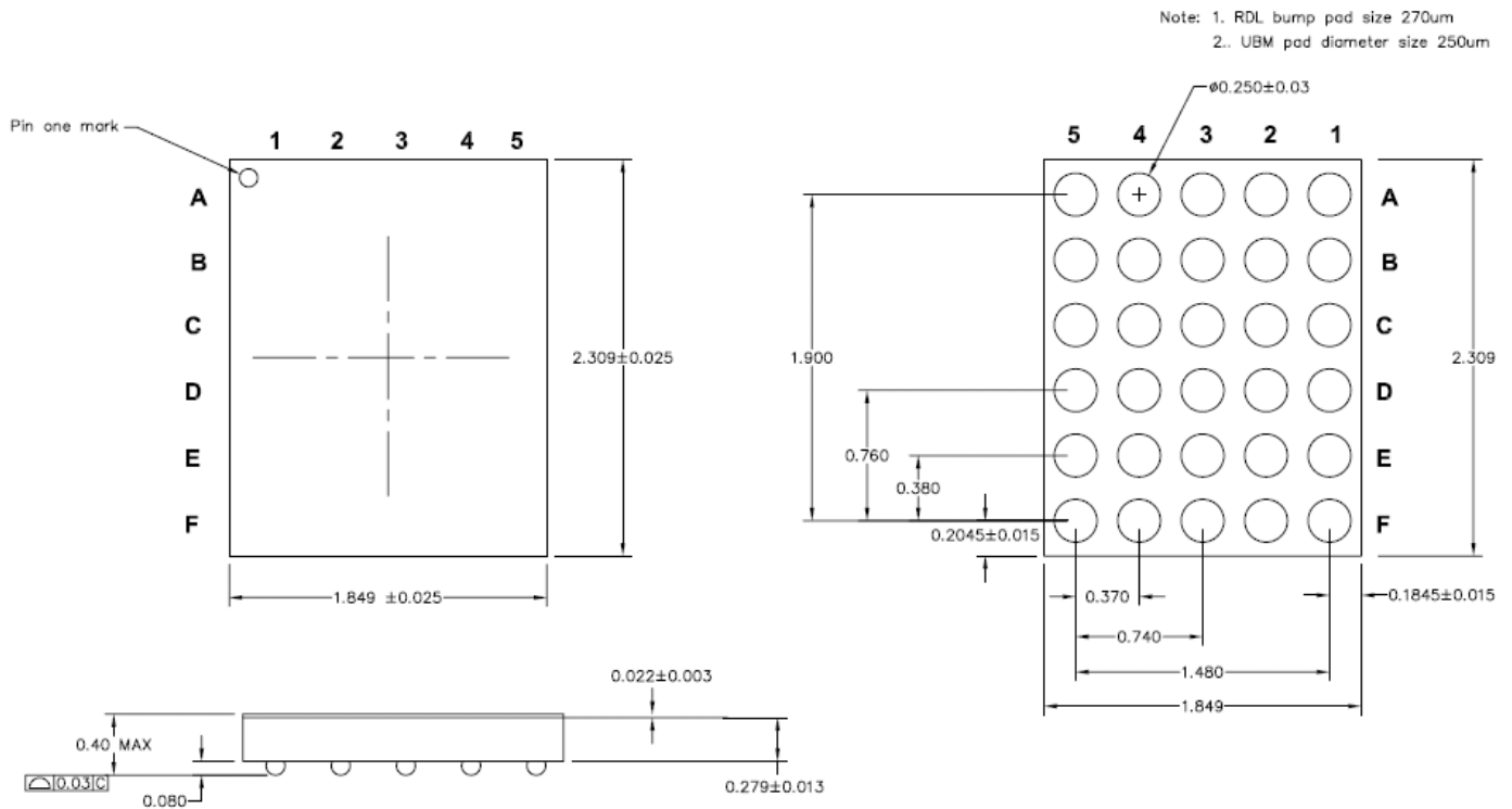
Figure 17. 30-Ball (1.85 x 2.31 x 0.40 mm) WLCSP
