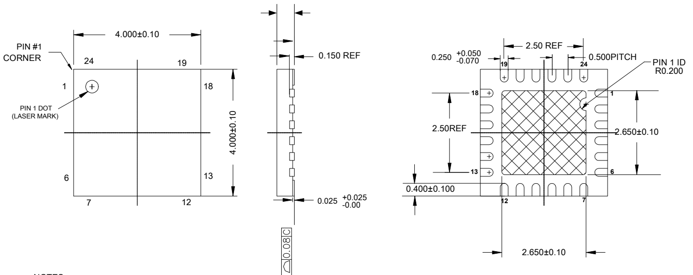
Figure 13. 24-Pin (4 x 4 x 0.55 mm) Sawn QFN
