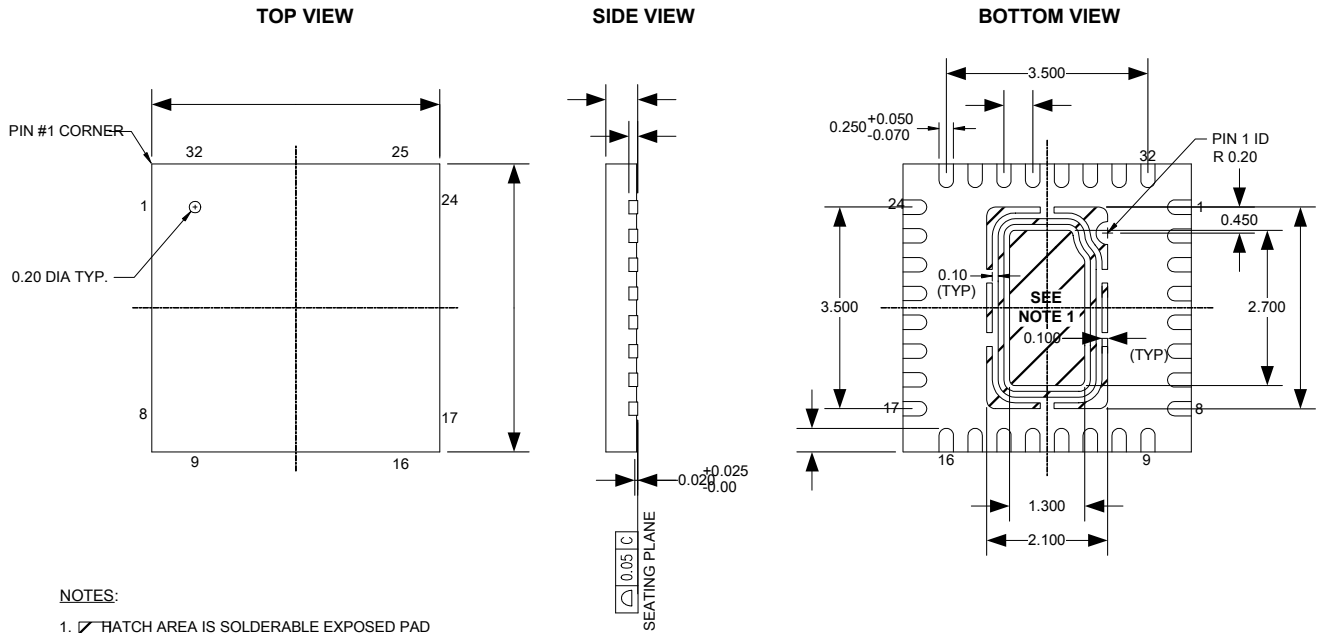
Figure 14. 32-Pin QFN 5 x 5 x 0.55 mm (Sawn)
