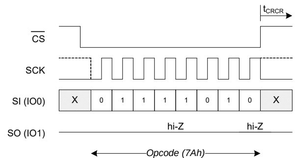
Figure 85. CRC Resume (EPCR) in SPI Mode
