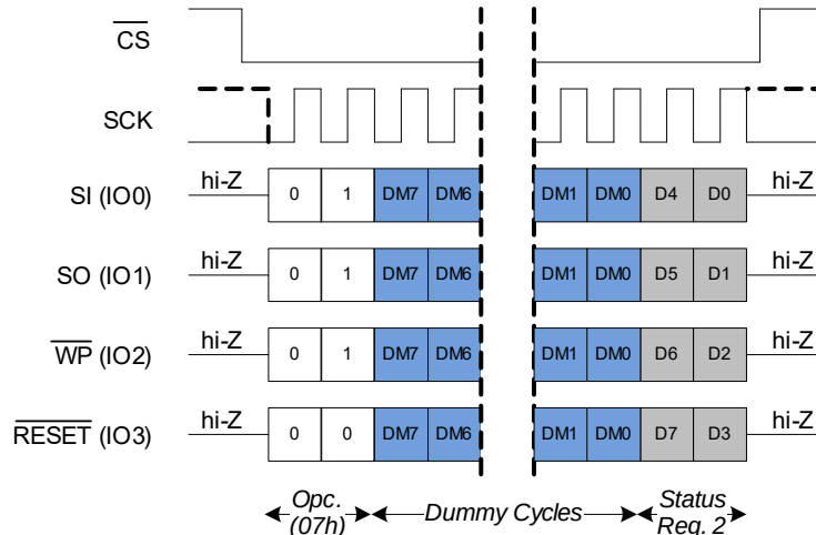
Figure 21. Read SR2 (RDSR2) in QPI Mode
