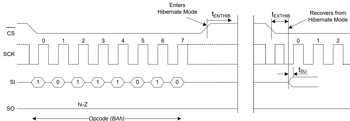
Figure 104. Hibernate Mode Operation in SPI Mode
