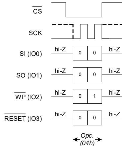
Figure 12. WRDI Bus Configuration in QPI Mode
