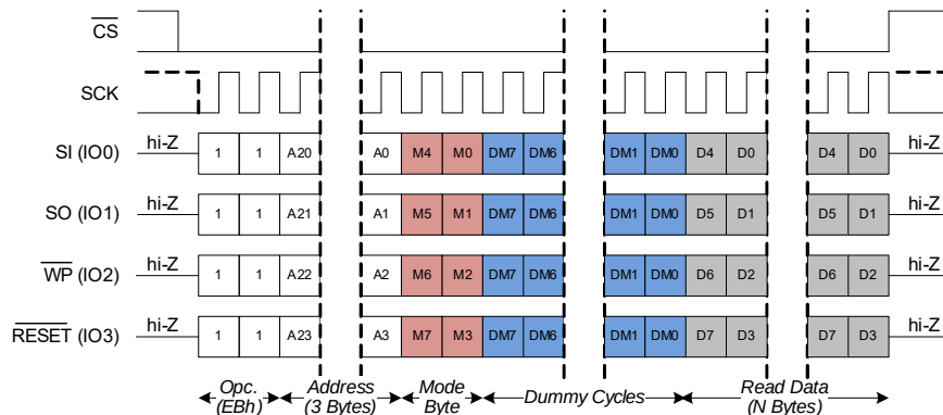
Figure 64. Quad I/O Read (QIOR) in QPI Mode
