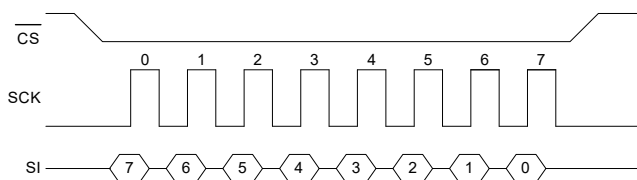
Figure 5. SPI Mode 0
