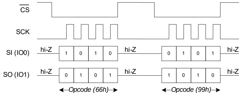
Figure 108. Software Reset Timing in DPI Mode
