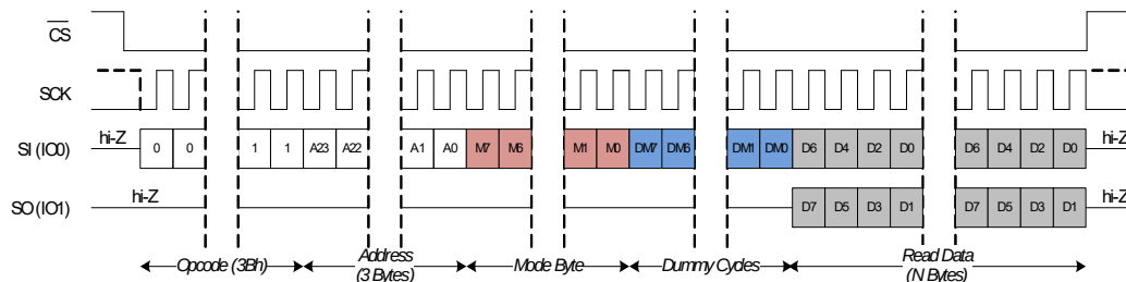
Figure 60. Double Output Read (DOR)
