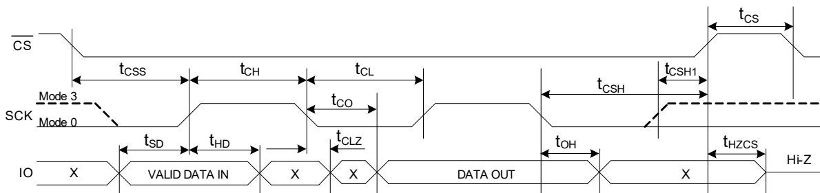
Figure 117. Chip Deselect ( \overline{CS} HIGH) - t_{CS} Timing
