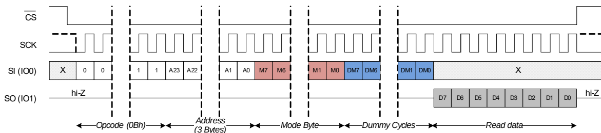
Figure 57. FAST_READ in DPI Mode
