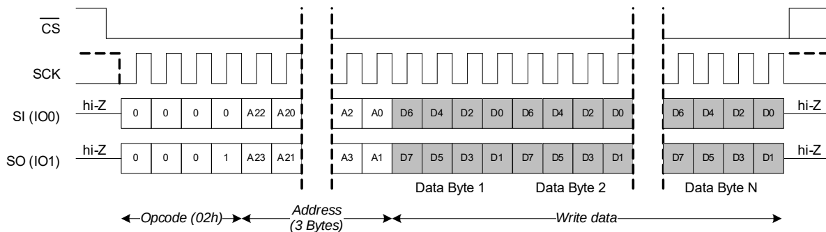
Figure 41. Memory Write (WRITE) in DPI Mode
