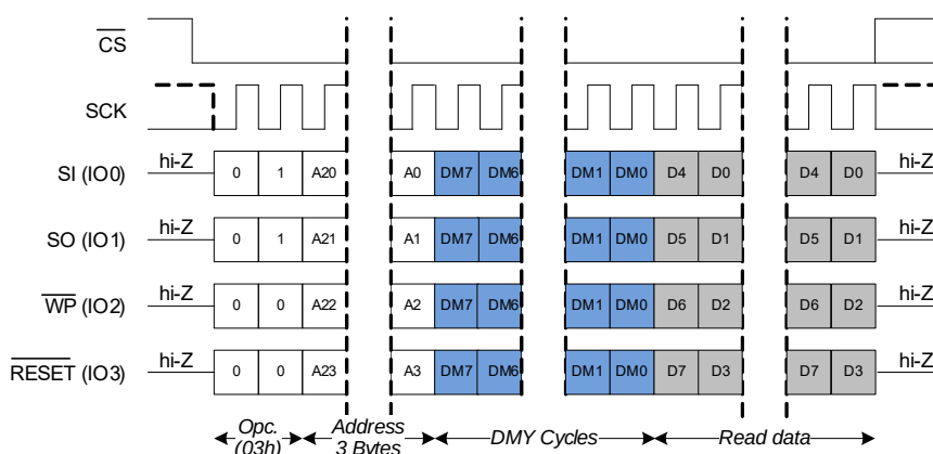
Figure 55. READ in QPI Mode
