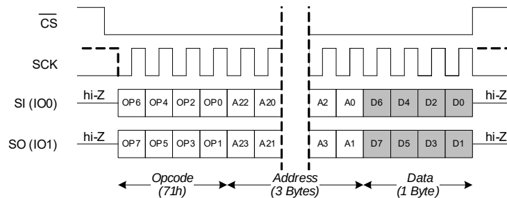
Figure 35. Write Any Register (WRAR) in DPI Mode
