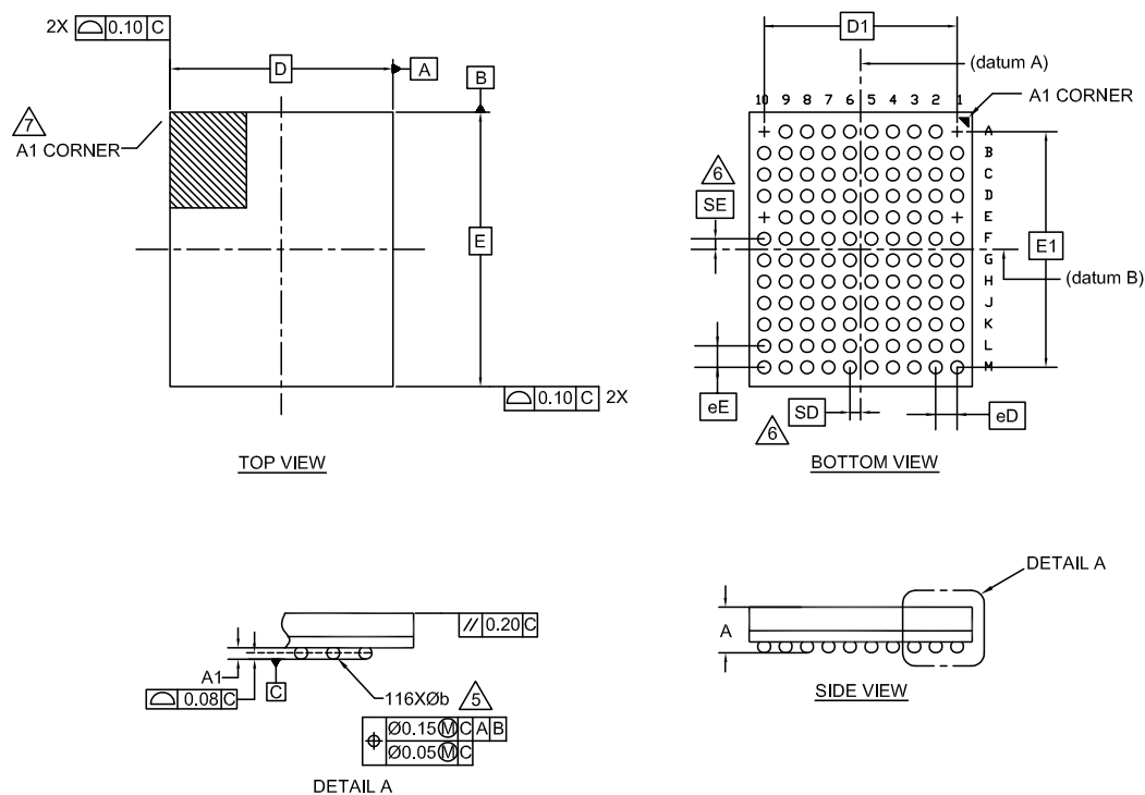
Figure 16. 116-BGA 5.2 × 6.4 × 0.70 mm
