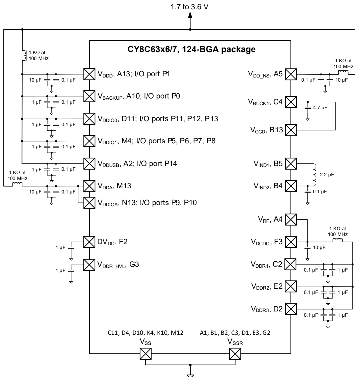
Figure 9. 124-BGA Power Connection Diagram
