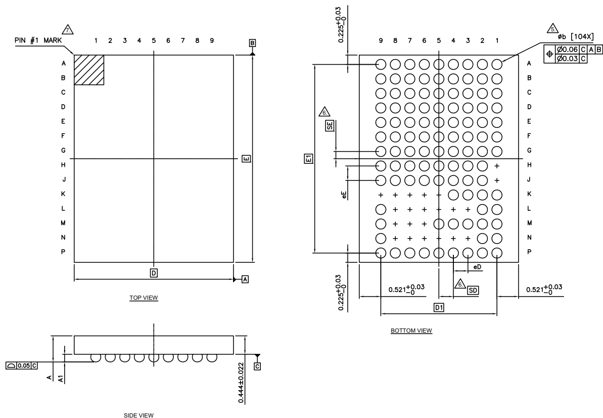
Figure 15. 104-WLCSP 3.8 × 5.0 × 0.65 mm
