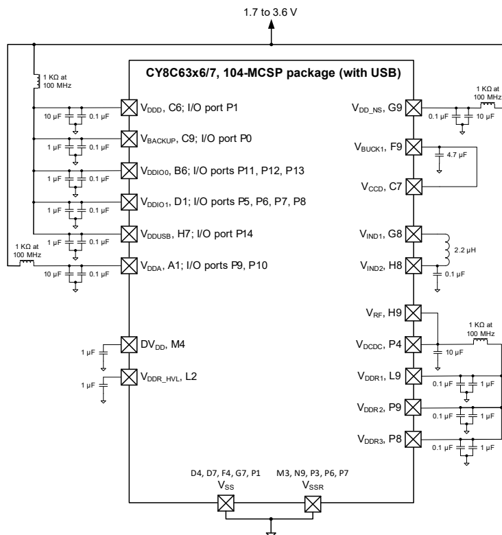
Figure 12. 104-MCSP-USB Power Connection Diagram
