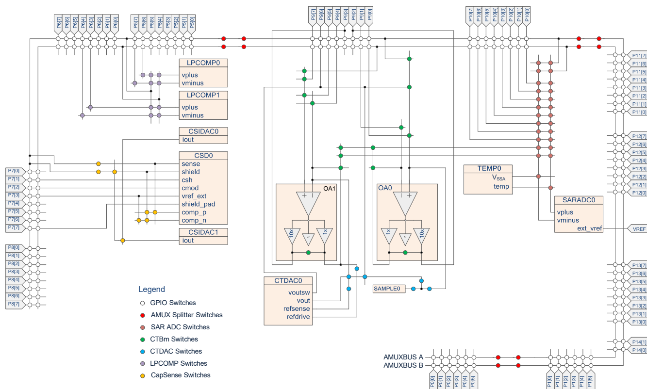
Figure 5. Analog Subsystem
