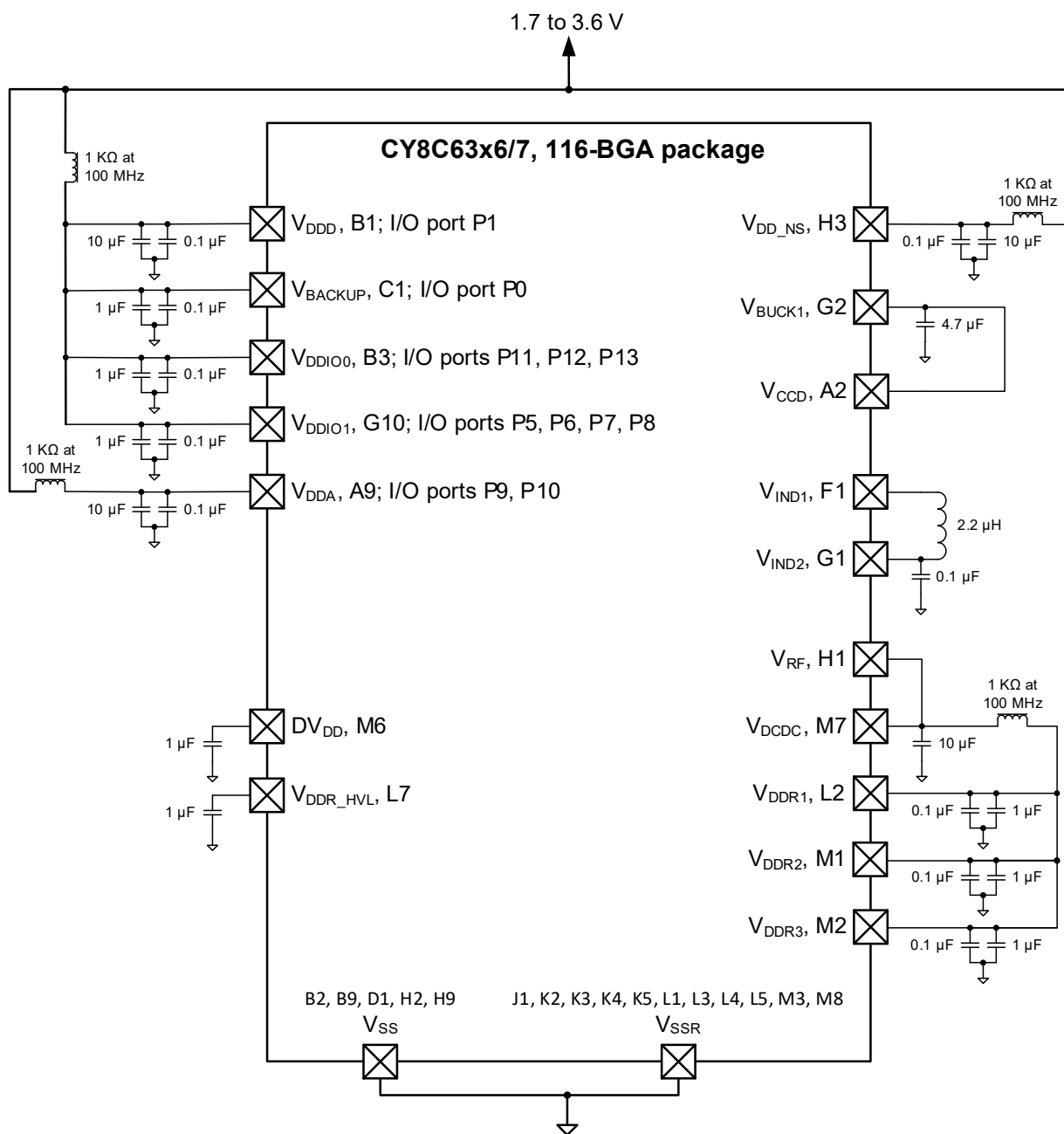
Figure 10. 116-BGA Power Connection Diagram
