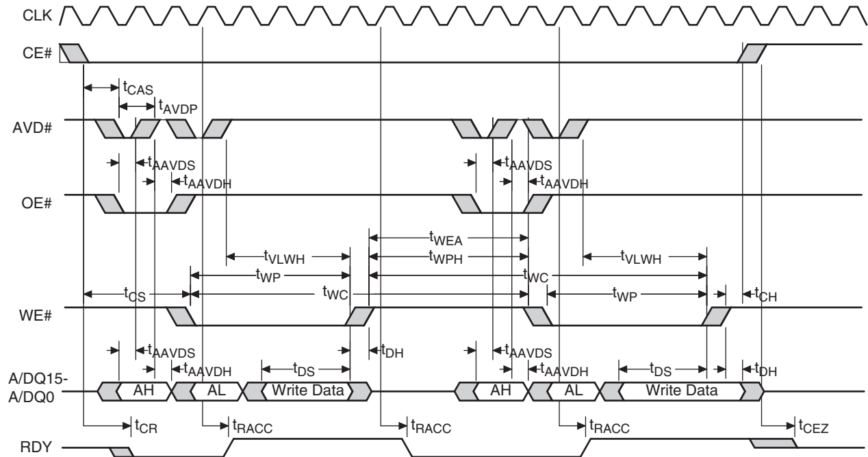
Figure 33. Synchronous Write Followed By Write - AADM Interface
