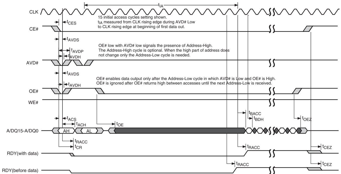
Figure 29. Synchronous Read Wrapped Burst - AADM Interface
