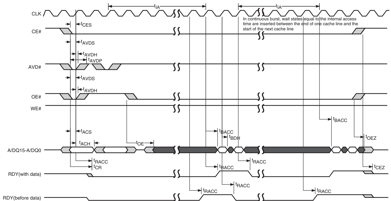
Figure 28. Synchronous Read Continuous Burst - AADM Interface
