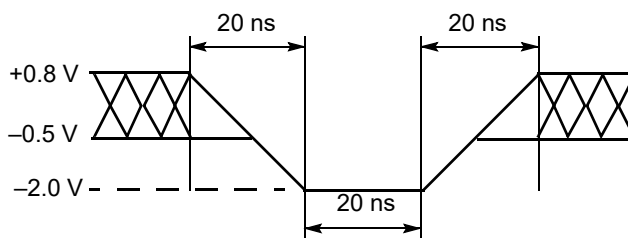
Figure 5. Maximum Negative Overshoot Waveform
