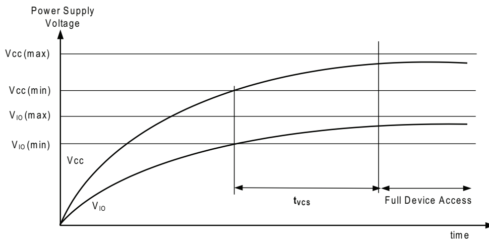
Figure 10. Power-up
