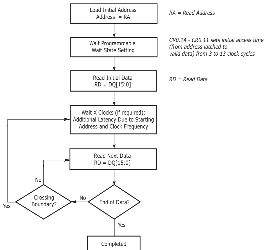
Figure 4. Synchronous Read
