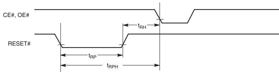
Figure 16. Reset Timings
