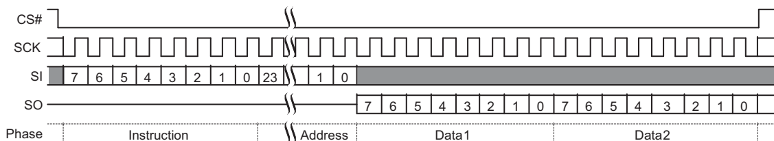
Figure 42. Read Data Command Sequence
