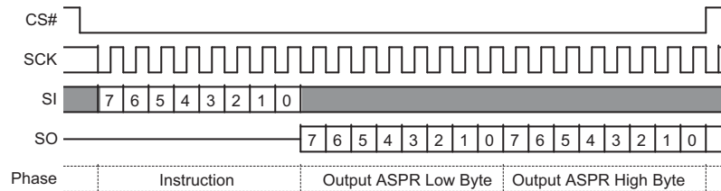
Figure 98. ASPRD Command
