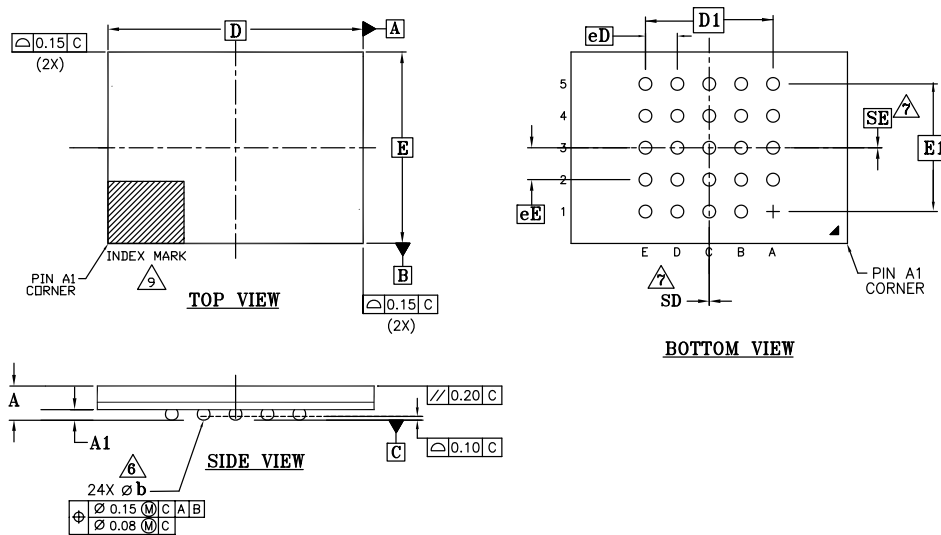
Figure 41. Ball Grid Array 24-Ball 6x8 mm (FAB024)
