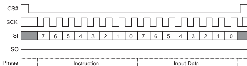
Figure 7. Single Bit Wide Input Command
