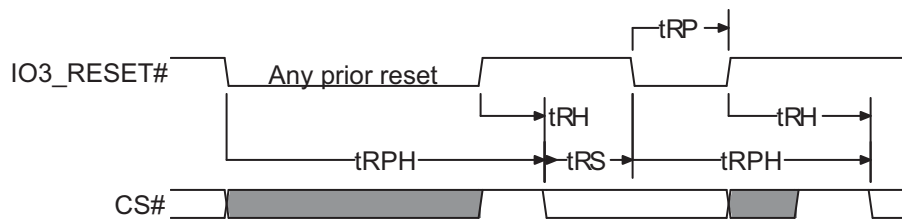
Figure 26. Hardware Reset when Quad Mode is not Enabled and IO3 / Reset# is Enabled
