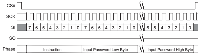
Figure 110. Password Program Command Sequence
