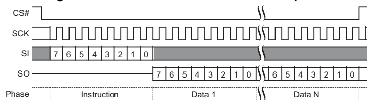
Figure 109. Password Read Command Sequence
