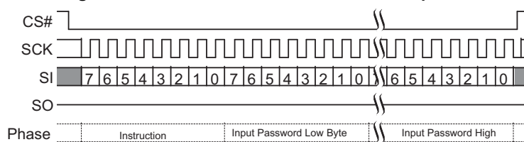
Figure 111. Password Unlock Command Sequence
