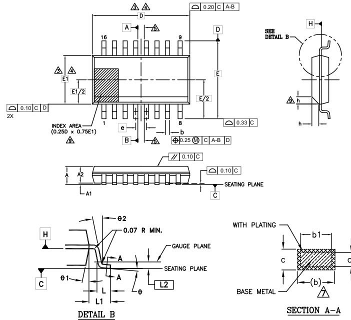
Figure 37. SOIC 16-Lead, 300-mil Body Width (SO3016)
