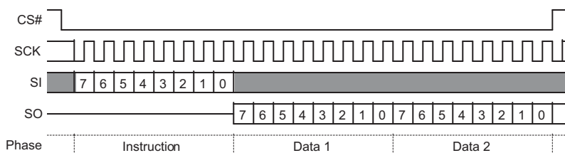
Figure 8. Single Bit Wide Output Command
