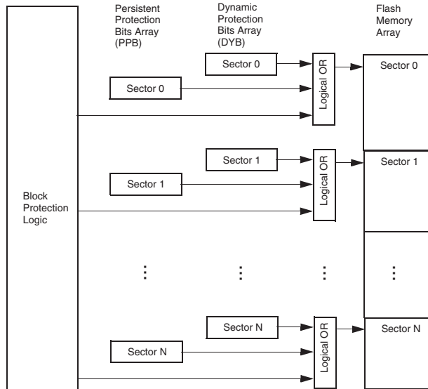
Figure 44. Advanced Sector Protection Overview
