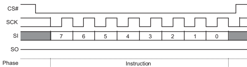
Figure 116. Deep Power-Down Command Sequence
