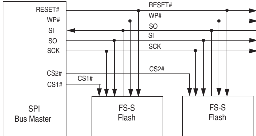
Figure 1. Bus Master and Memory Devices on the SPI Bus — Single Bit Data Path
