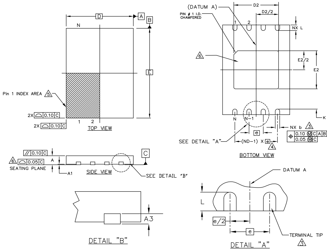
Figure 39. WSON 8-Contact 6x8 mm Leadless (WNH008)
