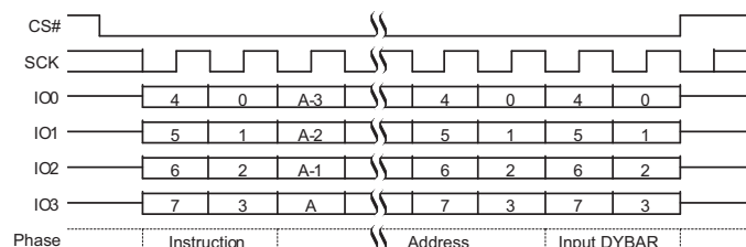
Figure 102. DYBWR Command Sequence
