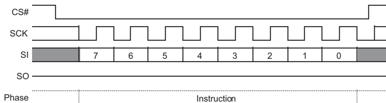
Figure 6. Stand Alone Instruction Command
