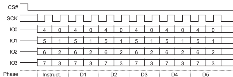
Figure 51. Read Status Register 1 (RDSR1) QPI Mode Command
