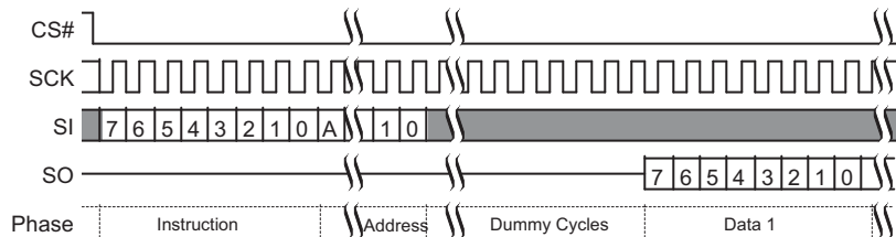
Figure 74. Fast Read (FAST_READ) Command Sequence (3-Byte Address, 0Bh [CR2V[7]=0])
