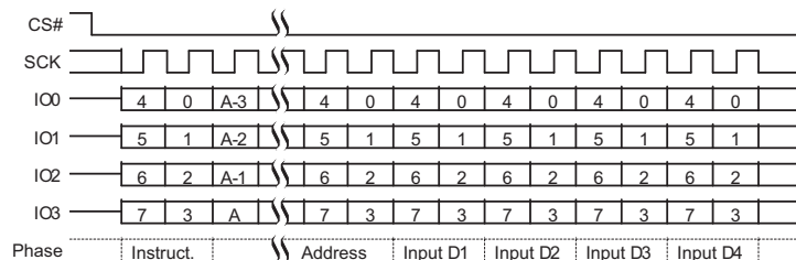
Figure 84. Page Program (PP 02h or 4PP 12h) QPI Mode Command Sequence
