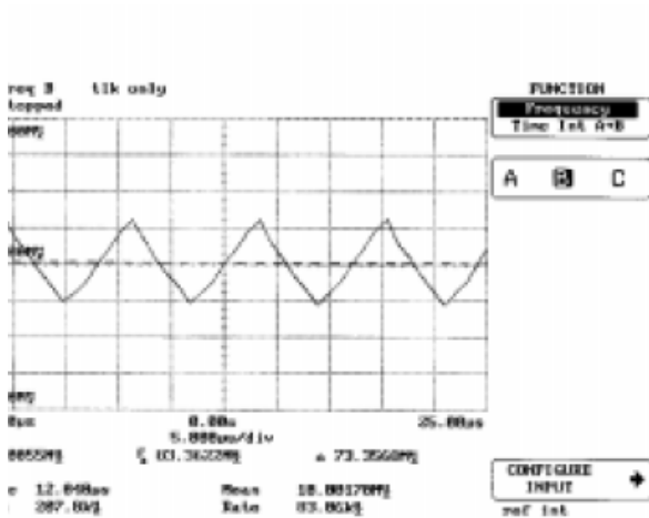
Figure 10. Frequency Modulation Profile
