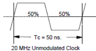
Figure 6. Perfect clock with no noise
