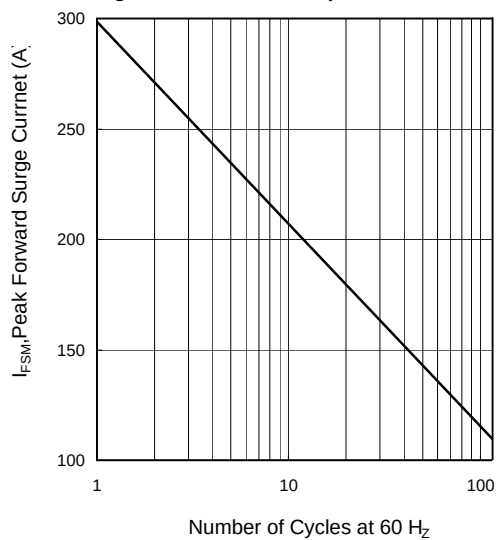
Fig. 6 - Maximum Non-repetitive Forward Surge
