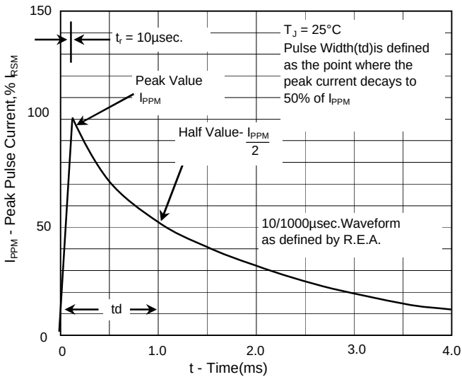
Fig. 3 - Pulse Waveform
