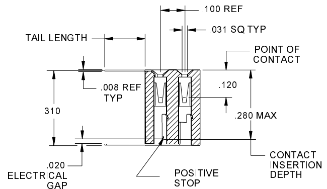
SECTION H-H
