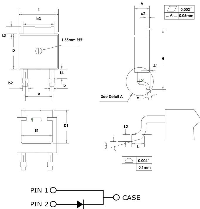
Package TO-252-2
