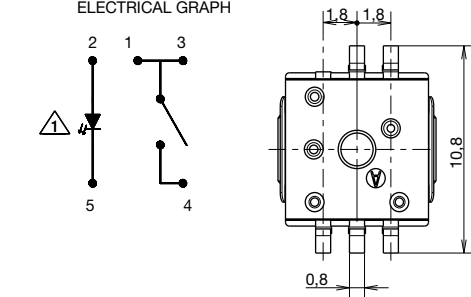
ELECTRICAL GRAPH
