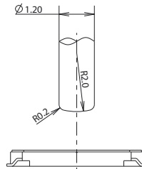
SET MAKER KNOB SIZE
