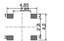
ALTERNATIVE PCB LAYOUT
