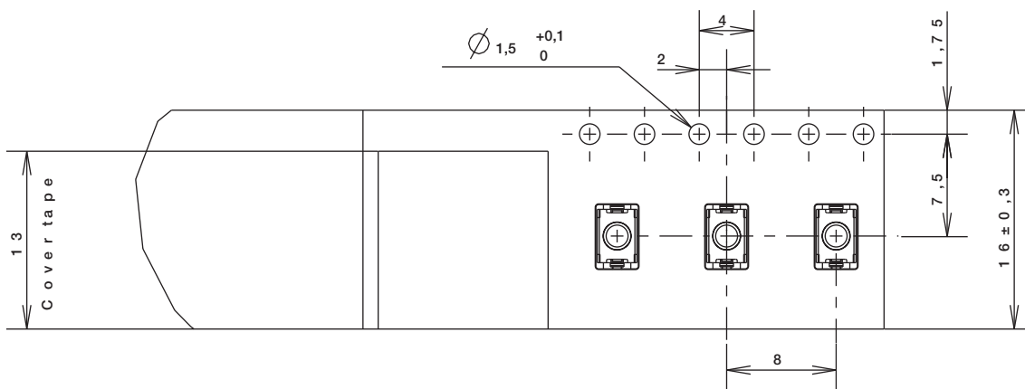
CARRIER TAPE
