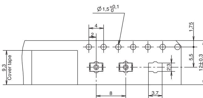
CARRIER TAPE
