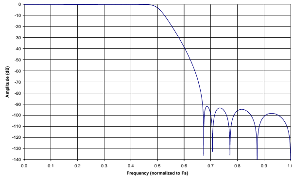
Figure 5. Double Speed Mode Stopband Rejection
