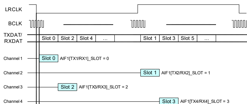
Figure 4-43. I 2 S Example
