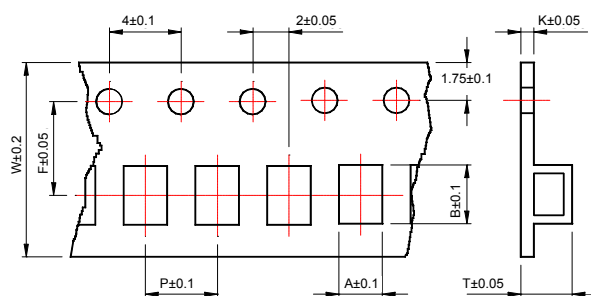
Tape Dimensions
