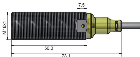
Fig. 26 Long body, flush version, cable
