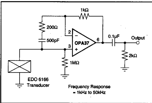
FIGURE 13. Hydrophone Preamplifier.
