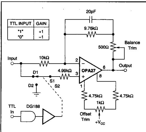
FIGURE 15. High Performance Synchronous Demodulator.
