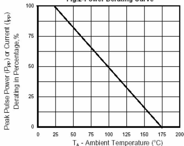
Fig.2-Power Derating Curve
